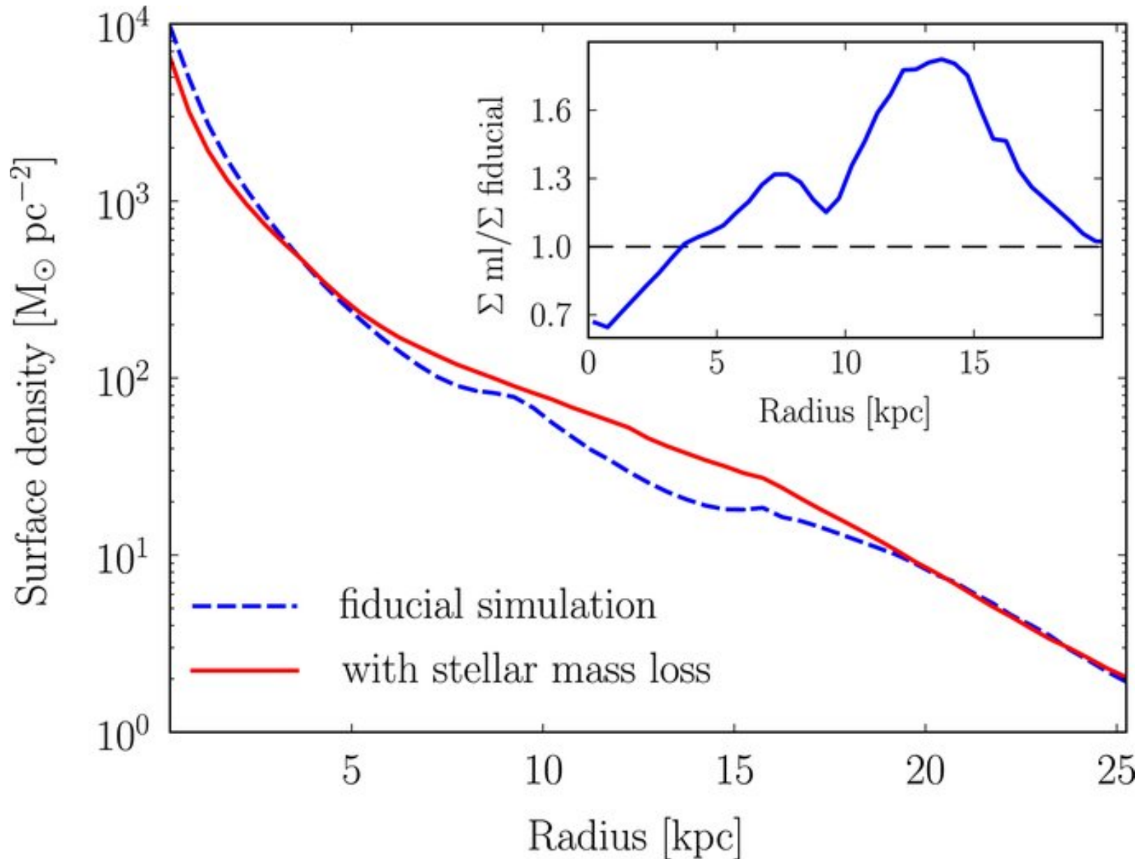
Figure 3. from Formation of Late-type Spiral Galaxies: Gas Return from Stellar Populations Regulates Disk Destruction and Bulge Growth MARTIG & BOURNAUD 2010 ApJL 714 L275 doi:10.1088/2041-8205/714/2/L275 https://dx.doi.org/10.1088/2041-8205/714/2/L275 © 2010. The American Astronomical Society. All rights reserved.
