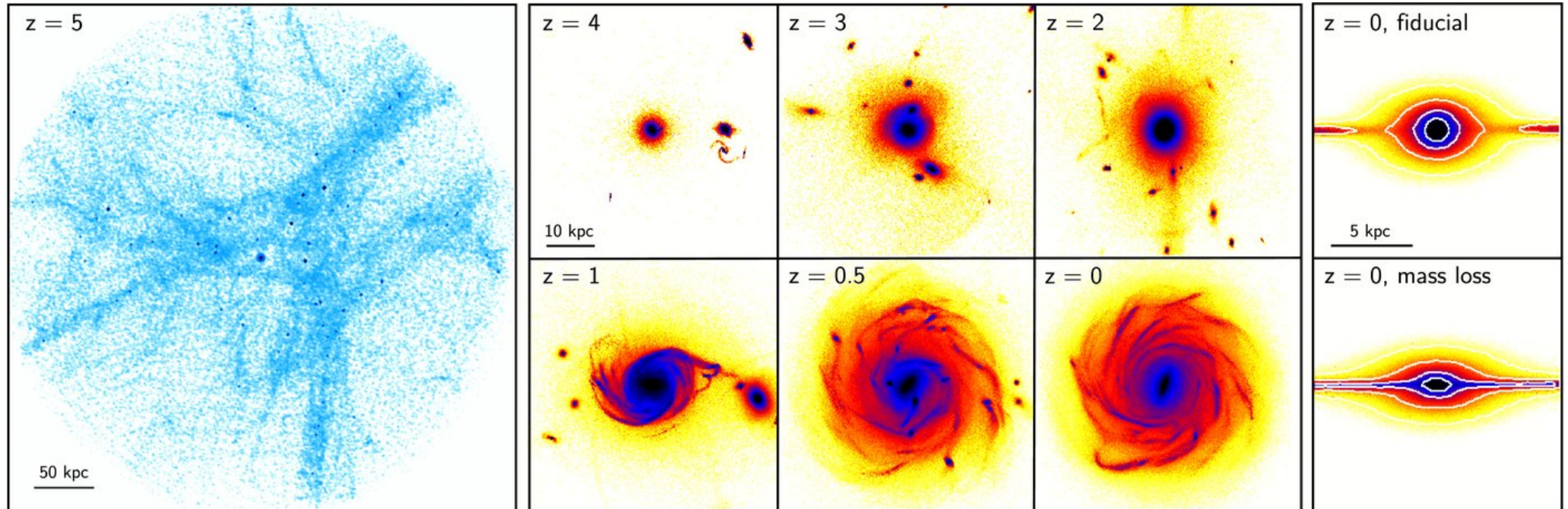
Figure 2. from Formation of Late-type Spiral Galaxies: Gas Return from Stellar Populations Regulates Disk Destruction and Bulge Growth MARTIG & BOURNAUD 2010 ApJL 714 L275 doi:10.1088/2041-8205/714/2/L275 https://dx.doi.org/10.1088/2041-8205/714/2/L275 © 2010. The American Astronomical Society. All rights reserved.
