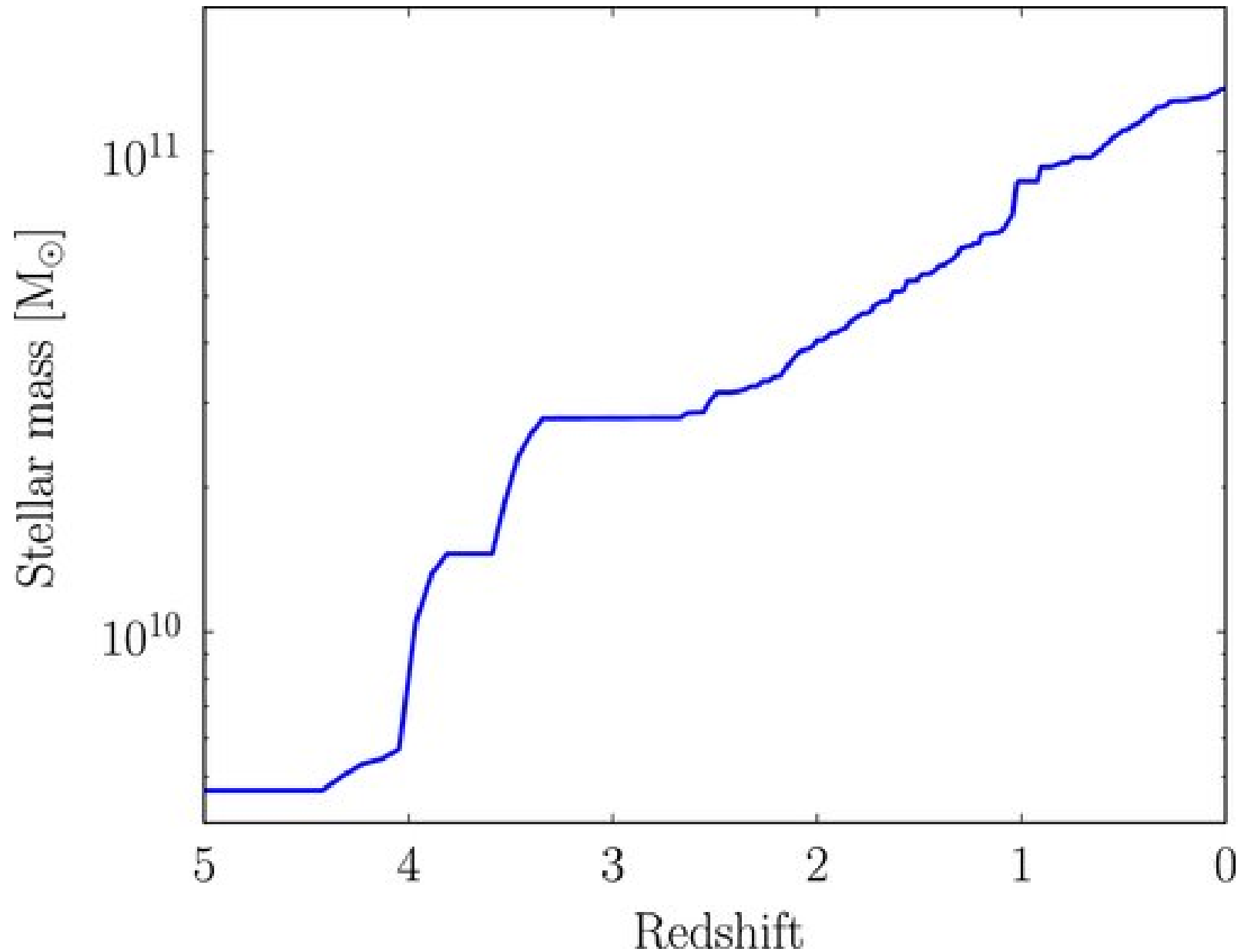
Figure 1. from Formation of Late-type Spiral Galaxies: Gas Return from Stellar Populations Regulates Disk Destruction and Bulge Growth MARTIG & BOURNAUD 2010 ApJL 714 L275 doi:10.1088/2041-8205/714/2/L275 https://dx.doi.org/10.1088/2041-8205/714/2/L275 © 2010. The American Astronomical Society. All rights reserved.
