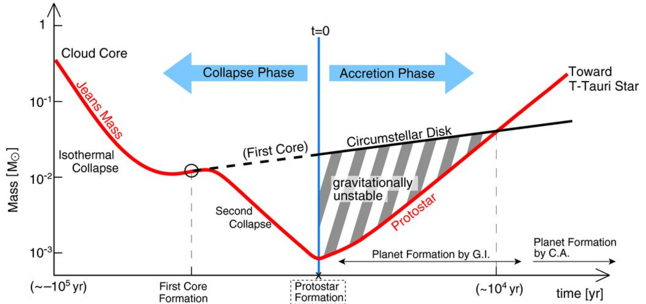
Figure 2. from Emergence of Protoplanetary Disks and Successive Formation of Gaseous Planets by Gravitational Instability INUTSUKA, MACHIDA, & MATSUMOTO 2010 ApJL 718 L58 doi:10.1088/2041-8205/718/2/L58 https://dx.doi.org/10.1088/2041-8205/718/2/L58 © 2010. The American Astronomical Society. All rights reserved.
