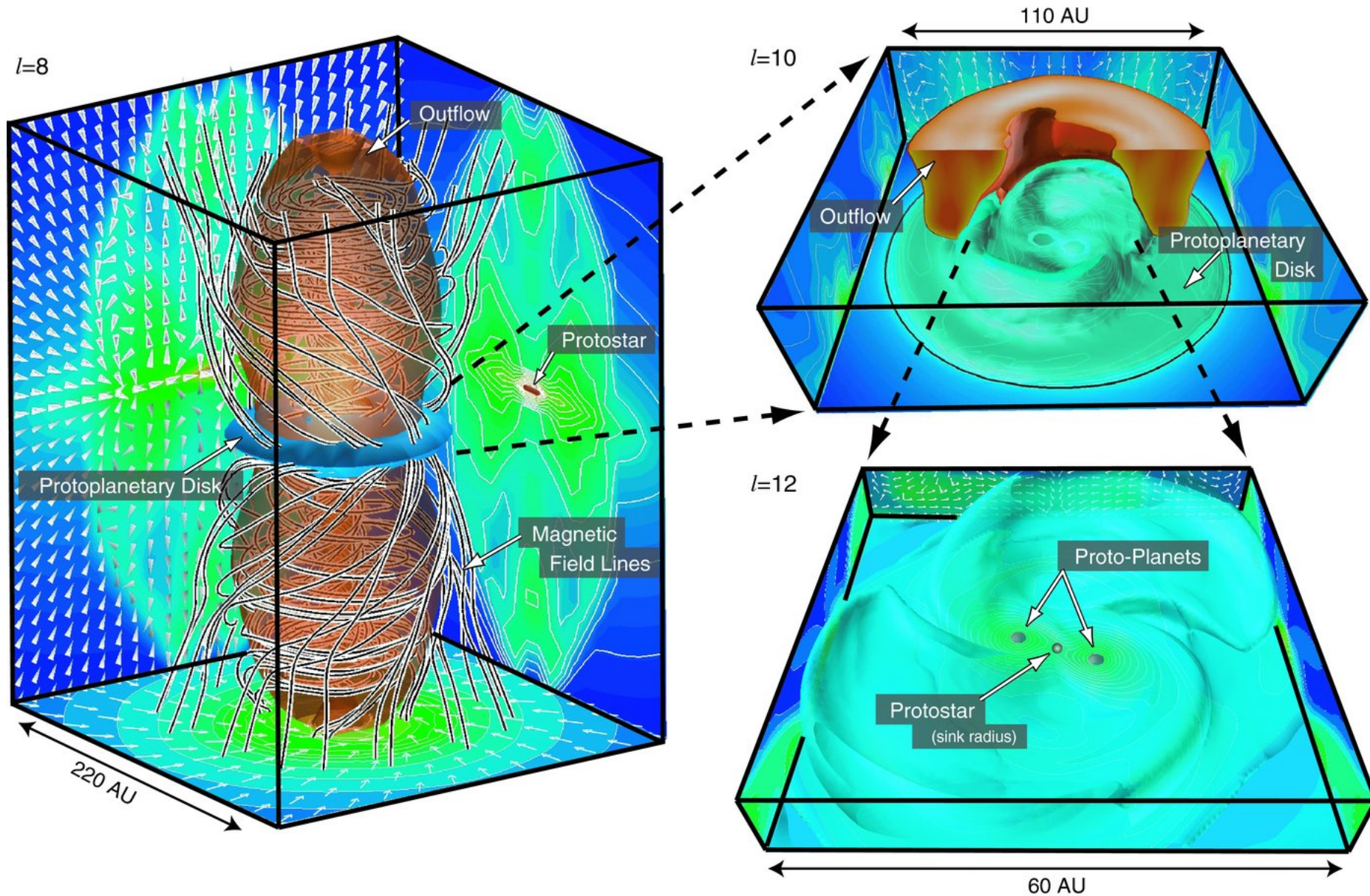
Figure 1. from Emergence of Protoplanetary Disks and Successive Formation of Gaseous Planets by Gravitational Instability INUTSUKA, MACHIDA, & MATSUMOTO 2010 ApJL 718 L58 doi:10.1088/2041-8205/718/2/L58 https://dx.doi.org/10.1088/2041-8205/718/2/L58 © 2010. The American Astronomical Society. All rights reserved.
