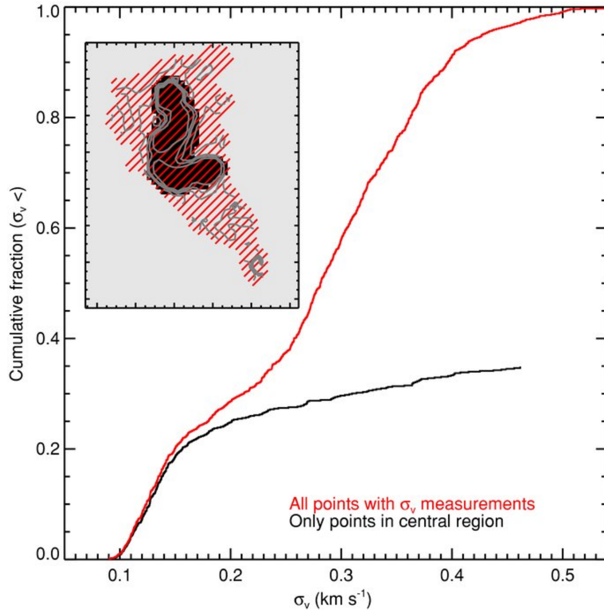
Figure 5. from Direct Observation of a Sharp Transition to Coherence in Dense Cores PINEDA ET AL. 2010 ApJL 712 L116 doi:10.1088/2041-8205/712/1/L116 https://dx.doi.org/10.1088/2041-8205/712/1/L116 © 2010. The American Astronomical Society. All rights reserved.
