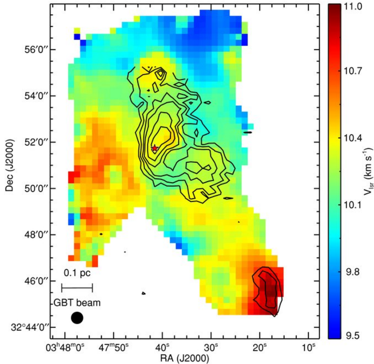
Figure 2. from Direct Observation of a Sharp Transition to Coherence in Dense Cores PINEDA ET AL. 2010 ApJL 712 L116 doi:10.1088/2041-8205/712/1/L116 https://dx.doi.org/10.1088/2041-8205/712/1/L116 © 2010. The American Astronomical Society. All rights reserved.
