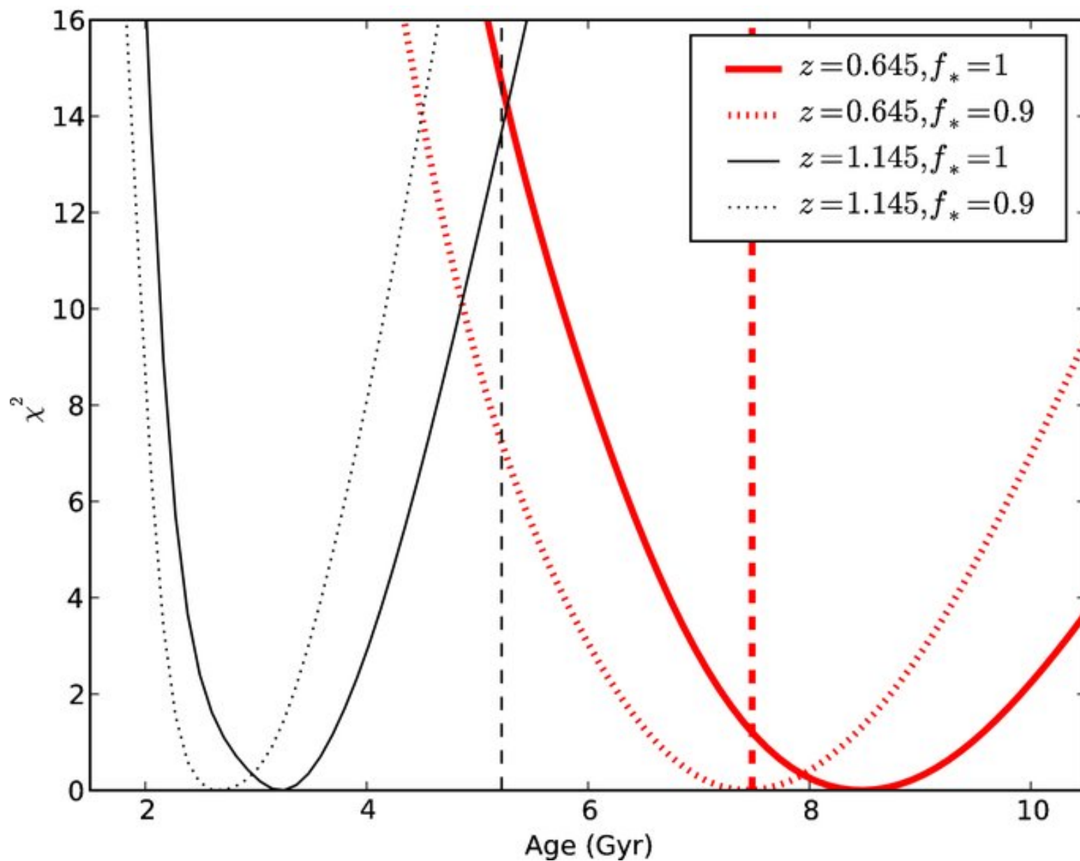
Figure 2. from Adaptive Optics Observations of B0128+437: A Low-mass, High-redshift Gravitational Lens LAGATTUTA, AUGER, & FASSNACHT 2010 ApJL 716 L185 doi:10.1088/2041-8205/716/2/L185 https://dx.doi.org/10.1088/2041-8205/716/2/L185
