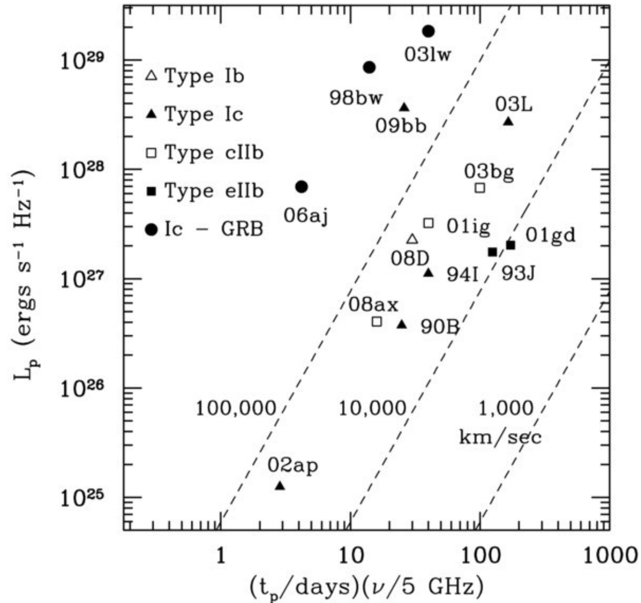
Figure 1. from Type IIb Supernovae with Compact and Extended Progenitors CHEVALIER & SODERBERG 2010 ApJL 711 L40 doi:10.1088/2041-8205/711/1/L40 https://dx.doi.org/10.1088/2041-8205/711/1/L40 © 2010. The American Astronomical Society. All rights reserved.
