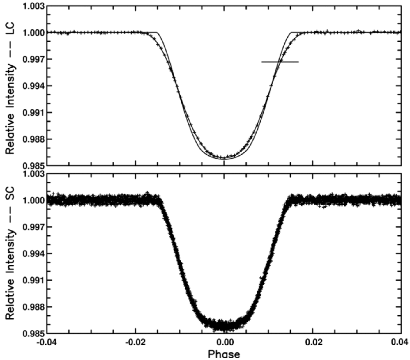
Figure 4. from Initial Characteristics of Kepler Short Cadence Data GILLILAND ET AL. 2010 ApJL 713 L160 doi:10.1088/2041-8205/713/2/L160 https://dx.doi.org/10.1088/2041-8205/713/2/L160 © 2010. The American Astronomical Society. All rights reserved.
