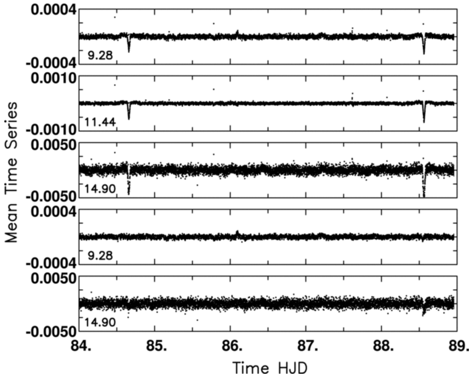
Figure 3. from Initial Characteristics of Kepler Short Cadence Data GILLILAND ET AL. 2010 ApJL 713 L160 doi:10.1088/2041-8205/713/2/L160 https://dx.doi.org/10.1088/2041-8205/713/2/L160 © 2010. The American Astronomical Society. All rights reserved.
