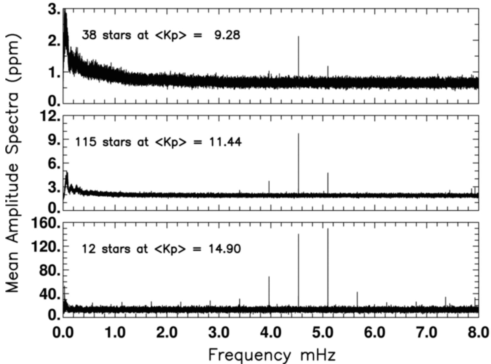
Figure 2. from Initial Characteristics of Kepler Short Cadence Data GILLILAND ET AL. 2010 ApJL 713 L160 doi:10.1088/2041-8205/713/2/L160 https://dx.doi.org/10.1088/2041-8205/713/2/L160 © 2010. The American Astronomical Society. All rights reserved.
