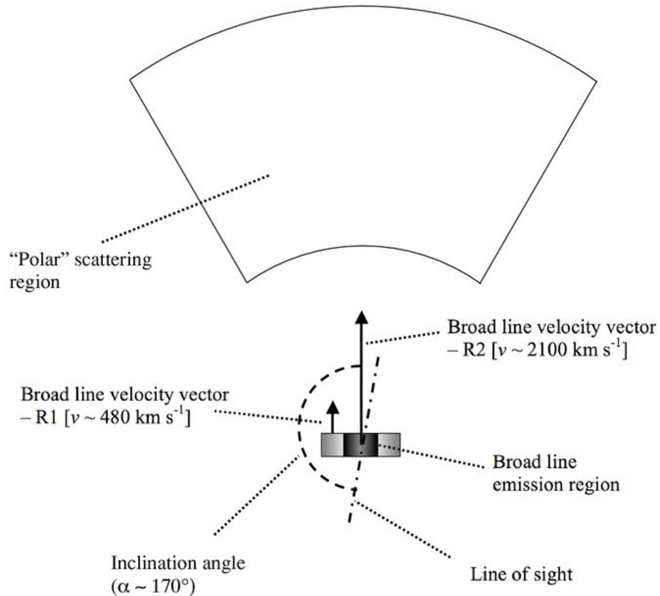
Figure 3. from Spectropolarimetric Evidence for a Kicked Supermassive Black Hole in the Quasar E1821+643 ROBINSON ET AL. 2010 ApJL 717 L122 doi:10.1088/2041-8205/717/2/L122 https://dx.doi.org/10.1088/2041-8205/717/2/L122 © 2010. The American Astronomical Society. All rights reserved.
