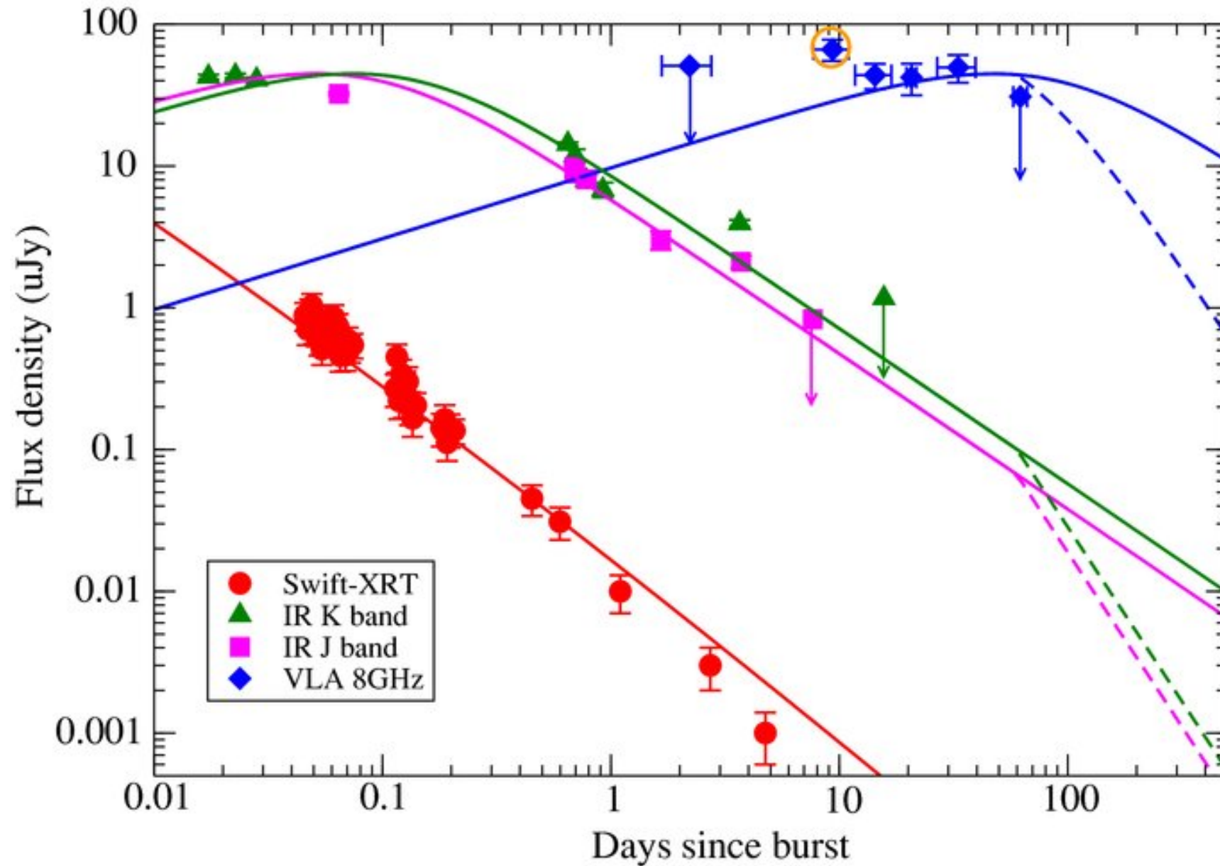
Figure 1. from Discovery of Radio Afterglow from the Most Distant Cosmic Explosion CHANDRA ET AL. 2010 ApJL 712 L31 doi:10.1088/2041-8205/712/1/L31 https://dx.doi.org/10.1088/2041-8205/712/1/L31 © 2010. The American Astronomical Society. All rights reserved.
