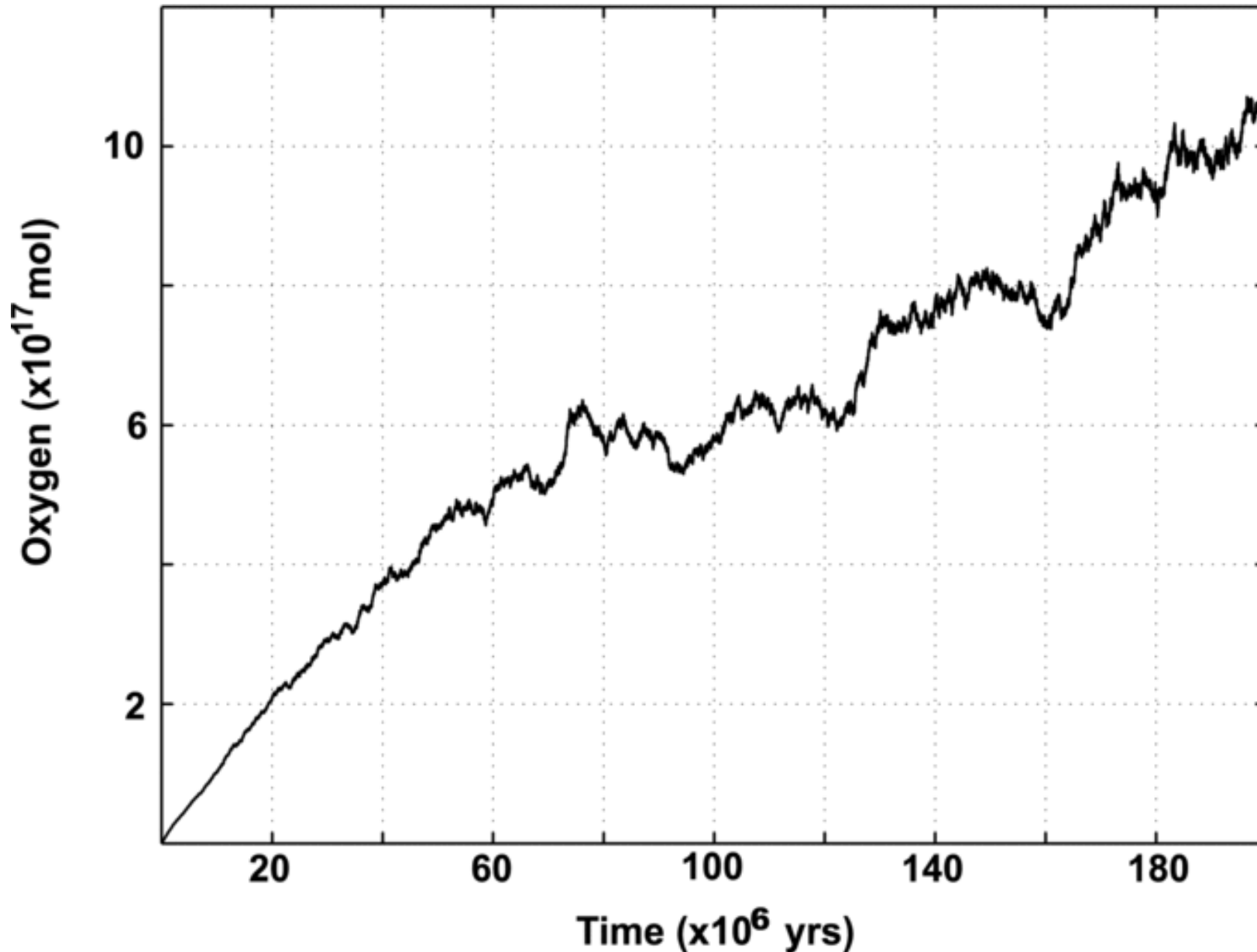
Figure 3. from The Great Oxidation of Earth's Atmosphere: Contesting the Yoyo Model Via Transition Stability Analysis CUNTZ, ROY, & MUSIELAK 2009 ApJ 706 L178 doi:10.1088/0004-637X/706/1/L178 https://dx.doi.org/10.1088/0004-637X/706/1/L178 © 2009. The American Astronomical Society. All rights reserved.
