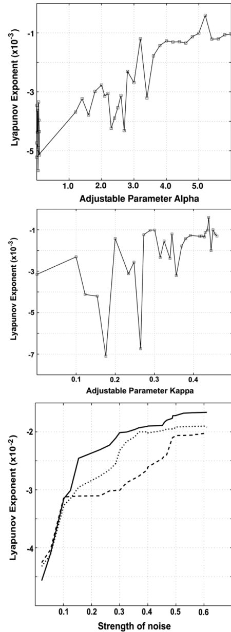
Figure 2. from The Great Oxidation of Earth's Atmosphere: Contesting the Yoyo Model Via Transition Stability Analysis CUNTZ, ROY, & MUSIELAK 2009 ApJ 706 L178 doi:10.1088/0004-637X/706/1/L178 https://dx.doi.org/10.1088/0004-637X/706/1/L178 © 2009. The American Astronomical Society. All rights reserved.
