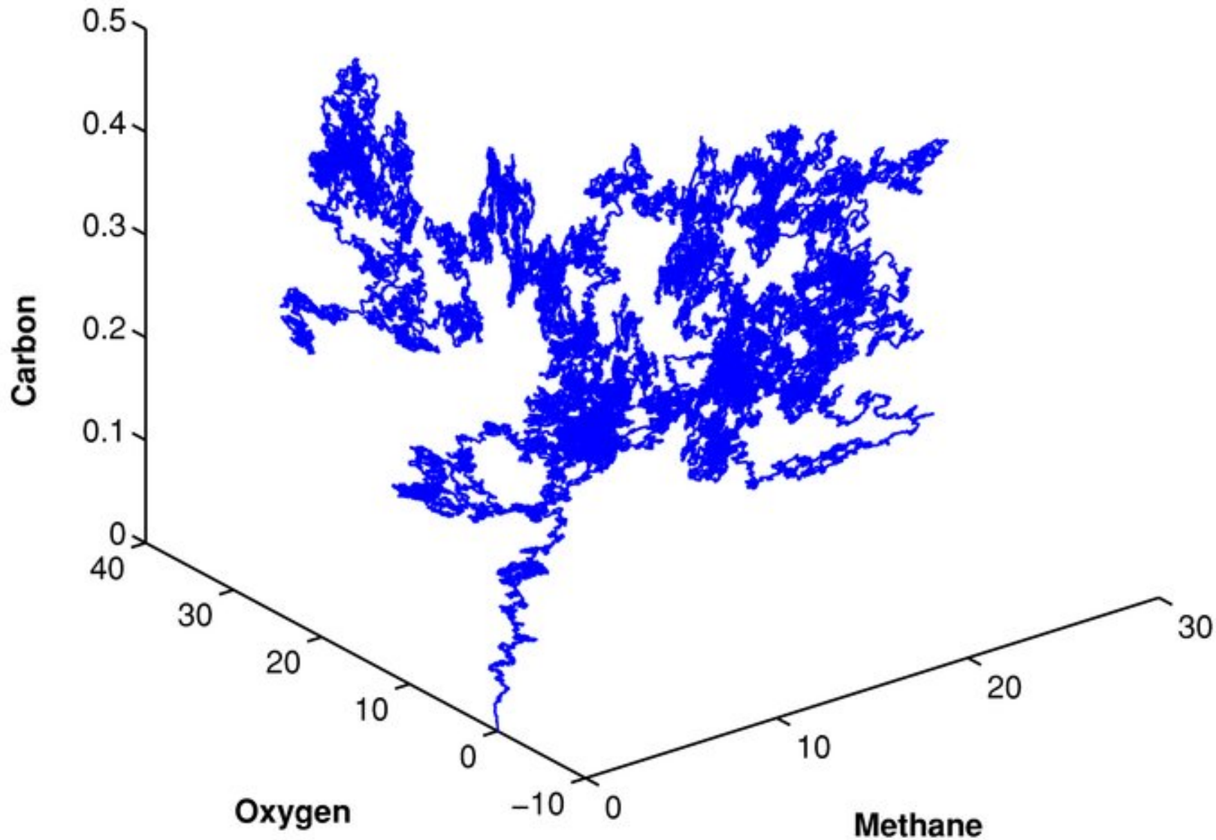
Figure 1. from The Great Oxidation of Earth's Atmosphere: Contesting the Yoyo Model Via Transition Stability Analysis CUNTZ, ROY, & MUSIELAK 2009 ApJ 706 L178 doi:10.1088/0004-637X/706/1/L178 https://dx.doi.org/10.1088/0004-637X/706/1/L178 © 2009. The American Astronomical Society. All rights reserved.
