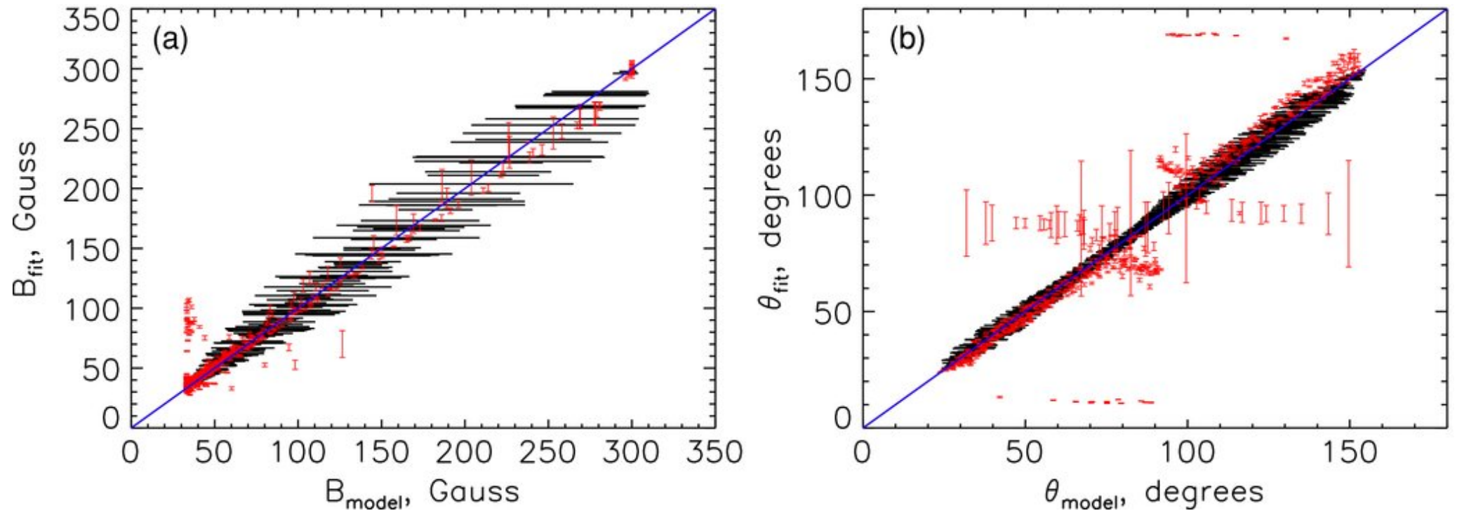
Figure 5. from Dynamic Magnetography of Solar Flaring Loops FLEISHMAN, NITA, & GARY 2009 ApJ 698 L183 doi:10.1088/0004-637X/698/2/L183 https://dx.doi.org/10.1088/0004-637X/698/2/L183 © 2009. The American Astronomical Society. All rights reserved.
