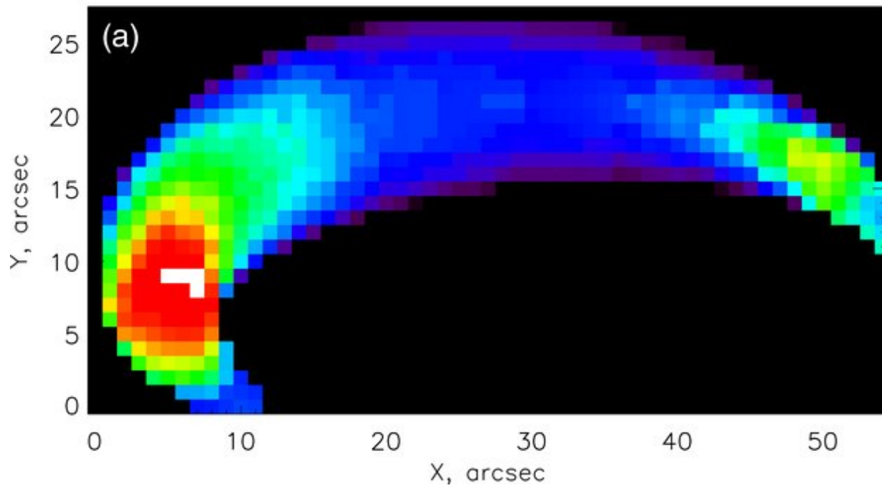
Figure 1. from Dynamic Magnetography of Solar Flaring Loops FLEISHMAN, NITA, & GARY 2009 ApJ 698 L183 doi:10.1088/0004-637X/698/2/L183 https://dx.doi.org/10.1088/0004-637X/698/2/L183 © 2009. The American Astronomical Society. All rights reserved.
