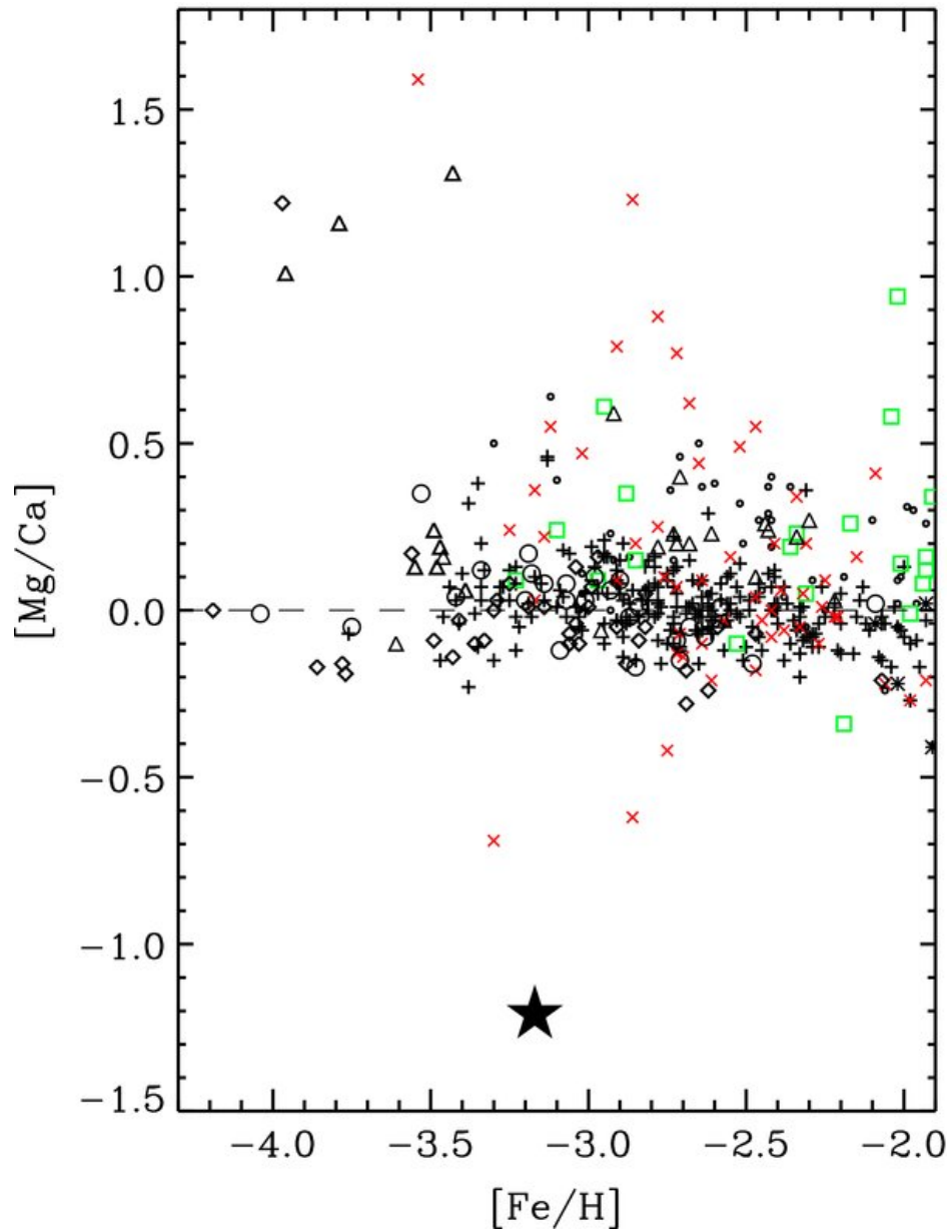
Figure 4. from A Unique Star in the Outer Halo of the Milky Way LAI ET AL. 2009 ApJ 697 L63 doi:10.1088/0004-637X/697/1/L63 https://dx.doi.org/10.1088/0004-637X/697/1/L63 © 2009. The American Astronomical Society. All rights reserved.
