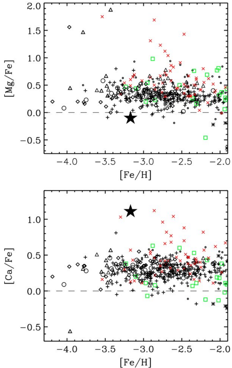
Figure 3. from A Unique Star in the Outer Halo of the Milky Way LAI ET AL. 2009 ApJ 697 L63 doi:10.1088/0004-637X/697/1/L63 https://dx.doi.org/10.1088/0004-637X/697/1/L63 © 2009. The American Astronomical Society. All rights reserved.
