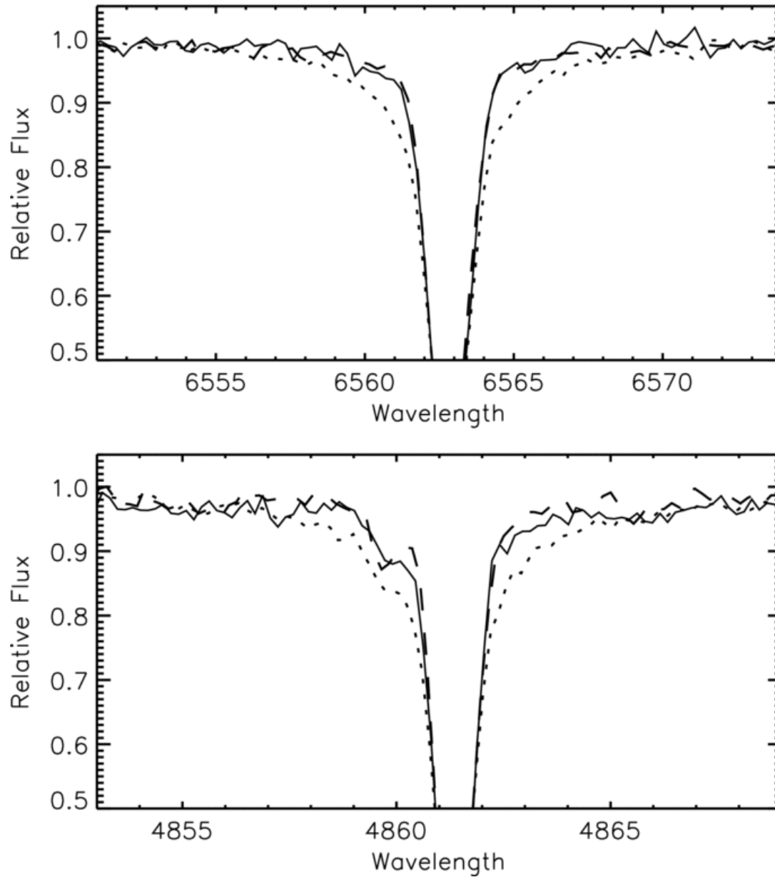
Figure 1. from A Unique Star in the Outer Halo of the Milky Way LAI ET AL. 2009 ApJ 697 L63 doi:10.1088/0004-637X/697/1/L63 https://dx.doi.org/10.1088/0004-637X/697/1/L63 © 2009. The American Astronomical Society. All rights reserved.
