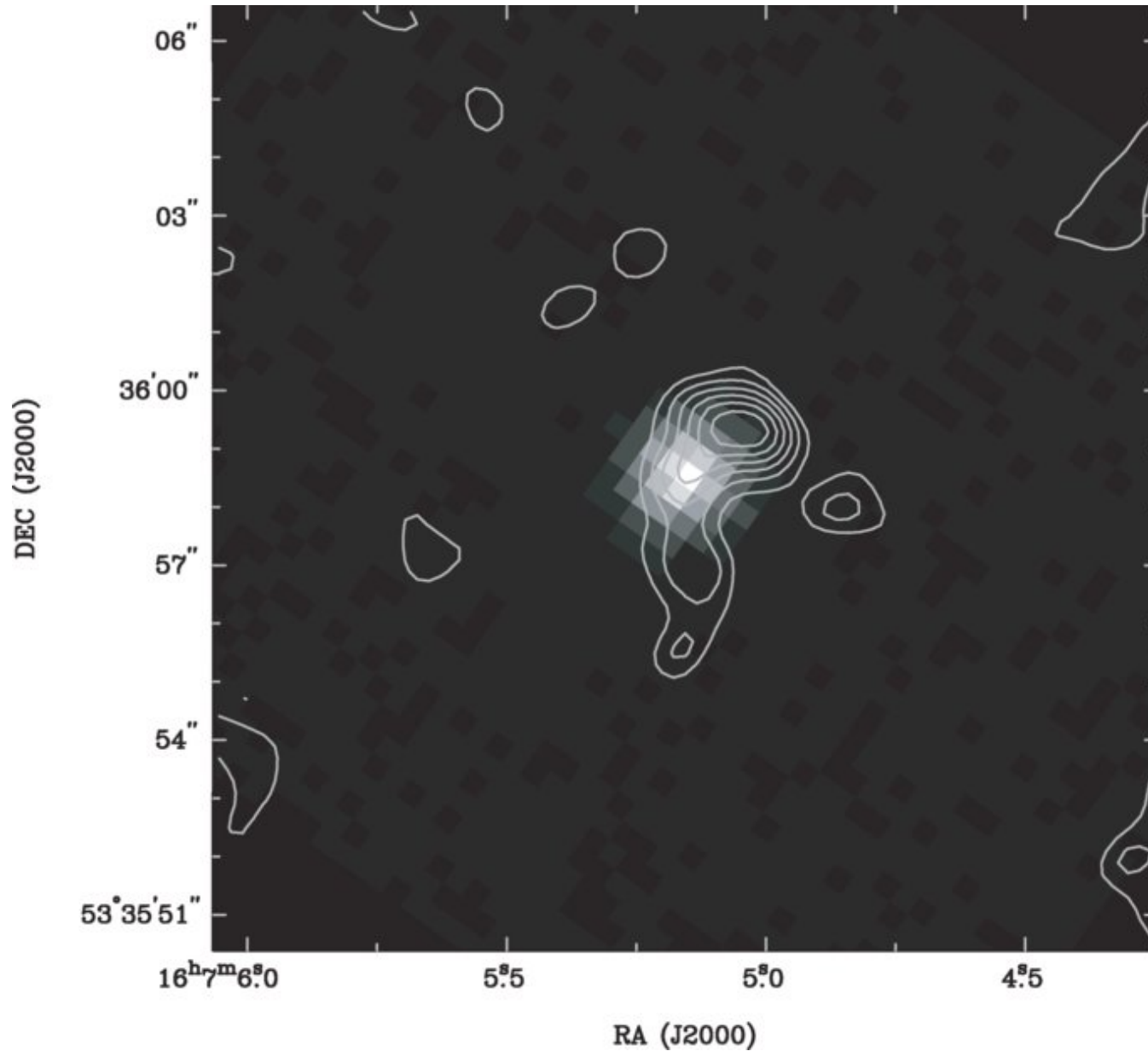
Figure 1. from Resolved Dust Emission in a Quasar at z = 3.65 CLEMENTS ET AL. 2009 ApJ 698 L188 doi:10.1088/0004-637X/698/2/L188 https://dx.doi.org/10.1088/0004-637X/698/2/L188 © 2009. The American Astronomical Society. All rights reserved.
