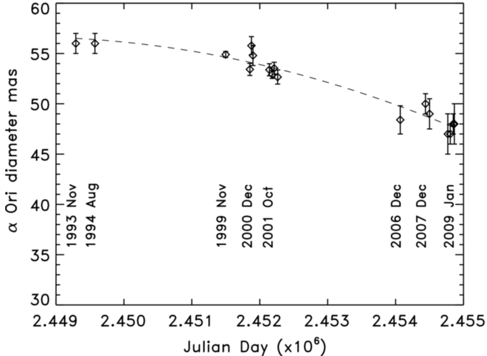
Figure 1. from A Systematic Change with Time in the Size of Betelgeuse TOWNES ET AL. 2009 ApJ 697 L127 doi:10.1088/0004-637X/697/2/L127 https://dx.doi.org/10.1088/0004-637X/697/2/L127 © 2009. The American Astronomical Society. All rights reserved.
