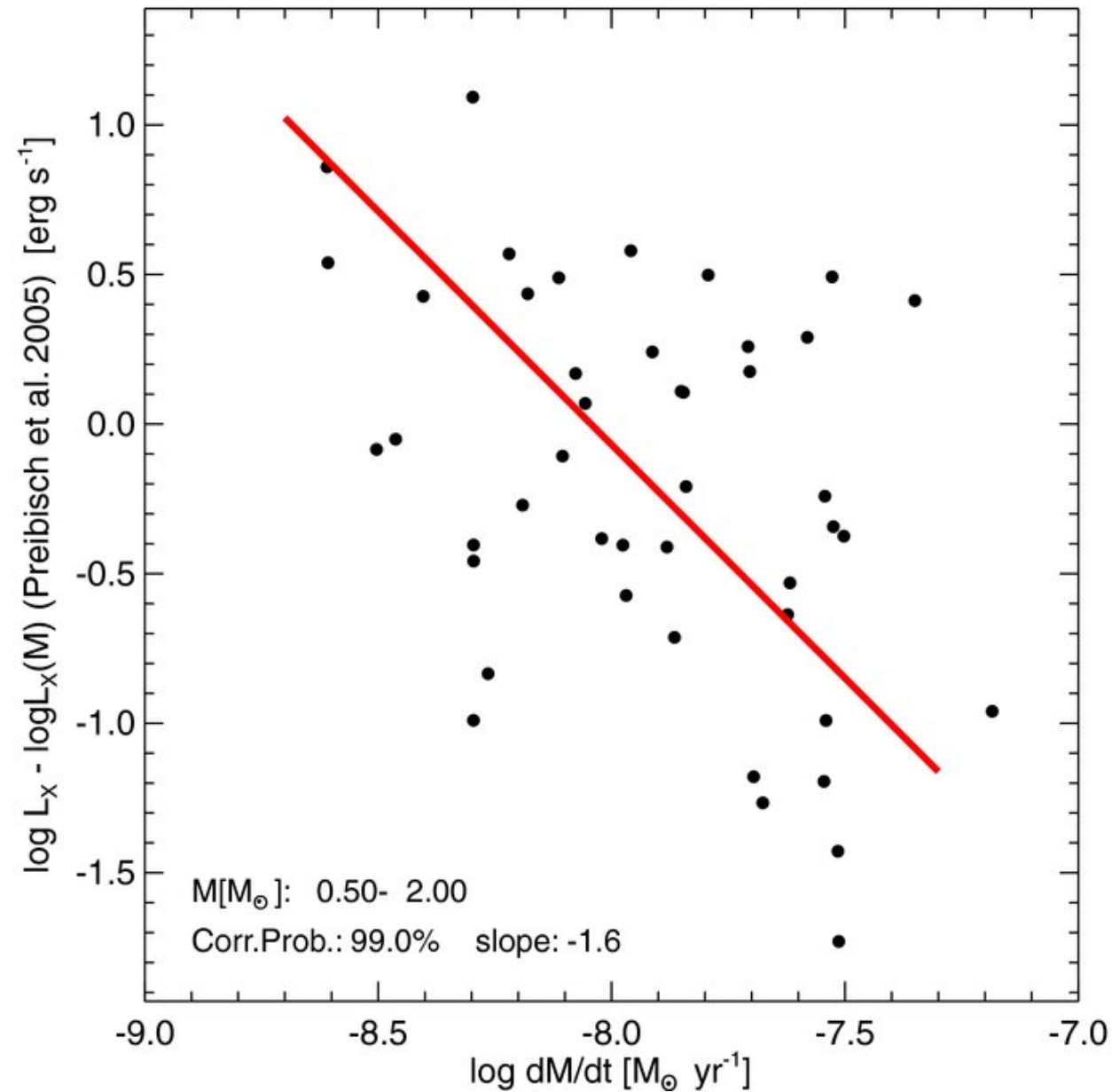
Figure 3. from X-ray Photoevaporation-Starved T Tauri Accretion DRAKE ET AL. 2009 ApJ 699 L35 doi:10.1088/0004-637X/699/1/L35 https://dx.doi.org/10.1088/0004-637X/699/1/L35 © 2009. The American Astronomical Society. All rights reserved.
