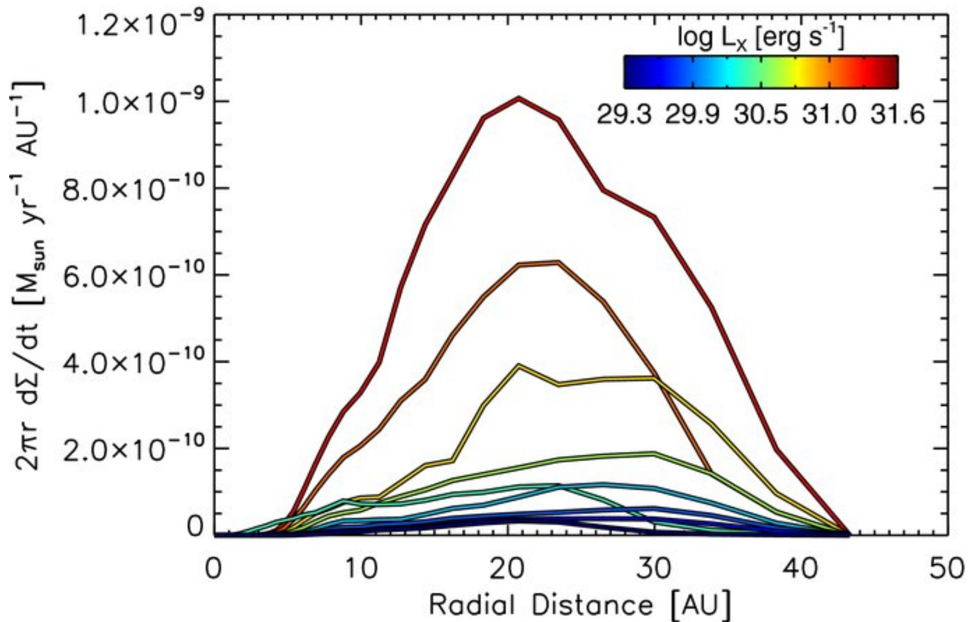
Figure 2. from X-ray Photoevaporation-Starved T Tauri Accretion DRAKE ET AL. 2009 ApJ 699 L35 doi:10.1088/0004-637X/699/1/L35 https://dx.doi.org/10.1088/0004-637X/699/1/L35 © 2009. The American Astronomical Society. All rights reserved.
