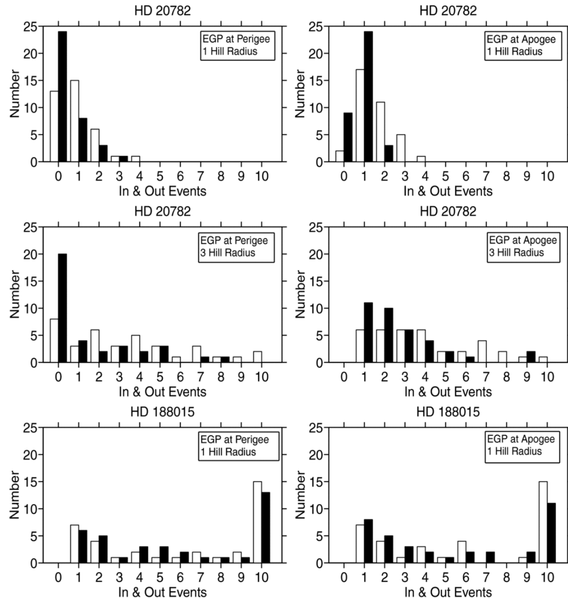
Figure 3. from On the Validity of the “Hill Radius Criterion” for the Ejection of Planets from Stellar Habitable Zones CUNTZ & YEAGER 2009 ApJ 697 L86 doi:10.1088/0004-637X/697/2/L86 https://dx.doi.org/10.1088/0004-637X/697/2/L86 © 2009. The American Astronomical Society. All rights reserved.
