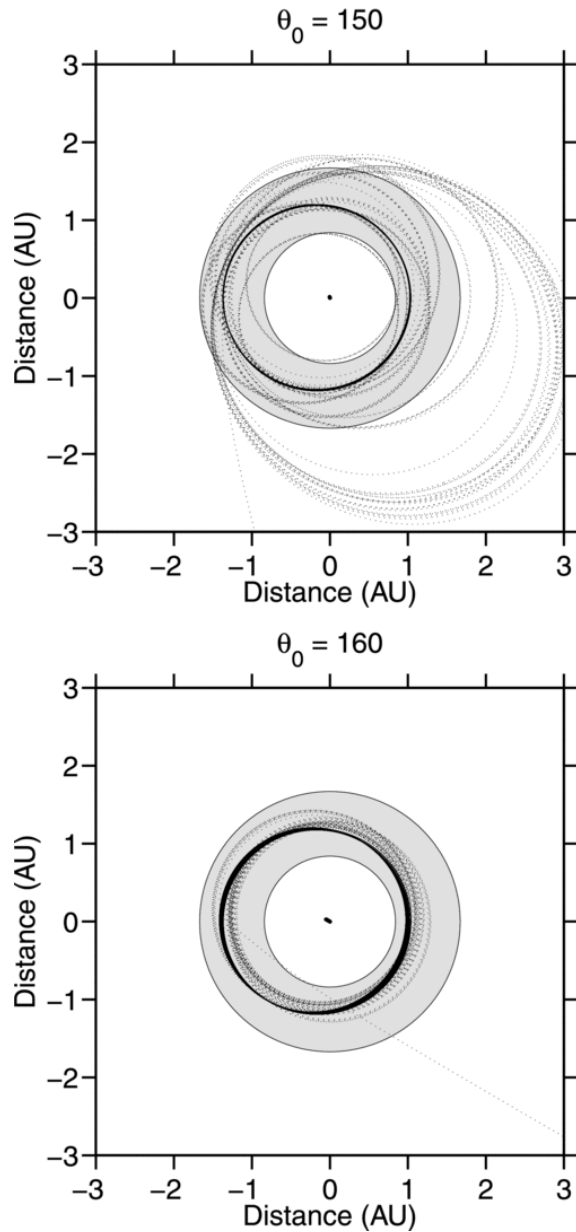
Figure 2. from On the Validity of the “Hill Radius Criterion” for the Ejection of Planets from Stellar Habitable Zones CUNTZ & YEAGER 2009 ApJ 697 L86 doi:10.1088/0004-637X/697/2/L86 https://dx.doi.org/10.1088/0004-637X/697/2/L86 © 2009. The American Astronomical Society. All rights reserved.
