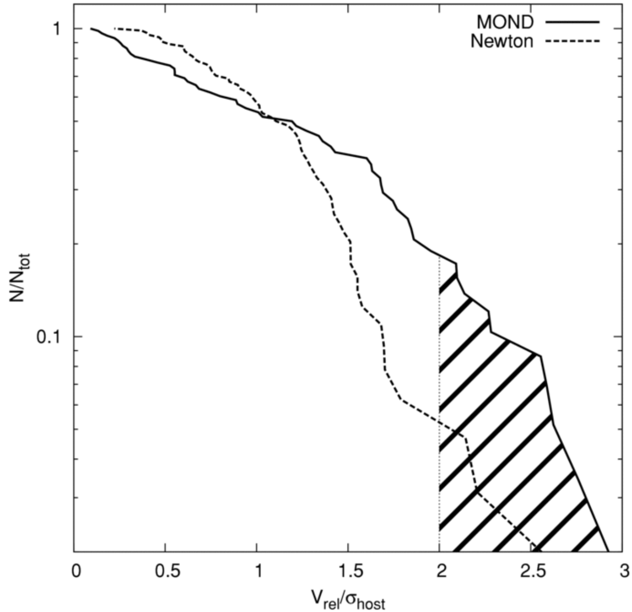
Figure 2. from Physics of Galactic Colliders: High-Speed Satellites in CDM Versus Mondian Cosmology LLINARES, ZHAO, & KNEBE 2009 ApJ 695 L145 doi:10.1088/0004-637X/695/2/L145 https://dx.doi.org/10.1088/0004-637X/695/2/L145 © 2009. The American Astronomical Society. All rights reserved.
