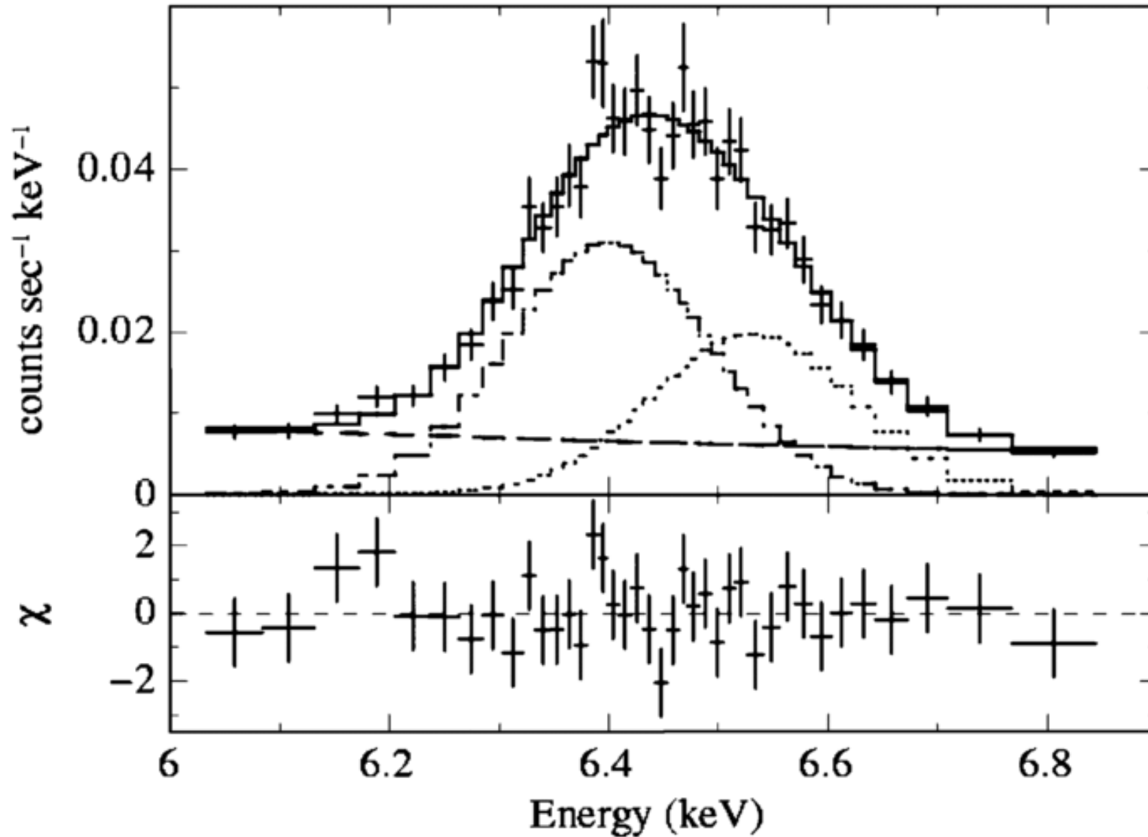
Figure 5. from Doppler-Broadened Iron X-Ray Lines From Tycho's Supernova Remnant FURUZAWA ET AL. 2009 ApJ 693 L61 doi:10.1088/0004-637X/693/2/L61 https://dx.doi.org/10.1088/0004-637X/693/2/L61 © 2009. The American Astronomical Society. All rights reserved.
