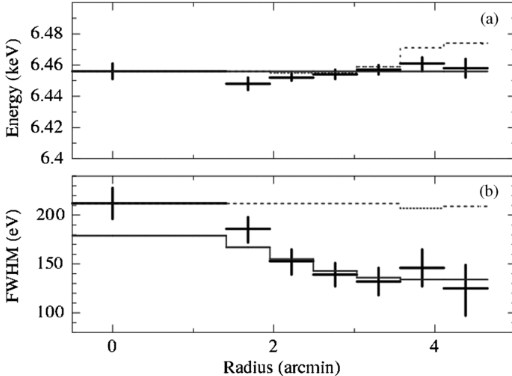
Figure 2. from Doppler-Broadened Iron X-Ray Lines From Tycho's Supernova Remnant FURUZAWA ET AL. 2009 ApJ 693 L61 doi:10.1088/0004-637X/693/2/L61 https://dx.doi.org/10.1088/0004-637X/693/2/L61 © 2009. The American Astronomical Society. All rights reserved.
