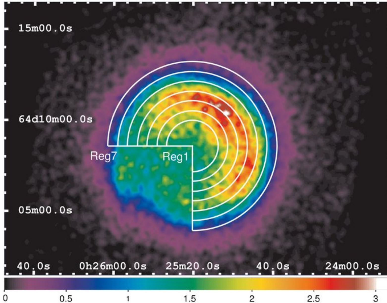
Figure 1. from Doppler-Broadened Iron X-Ray Lines From Tycho's Supernova Remnant FURUZAWA ET AL. 2009 ApJ 693 L61 doi:10.1088/0004-637X/693/2/L61 https://dx.doi.org/10.1088/0004-637X/693/2/L61 © 2009. The American Astronomical Society. All rights reserved.
