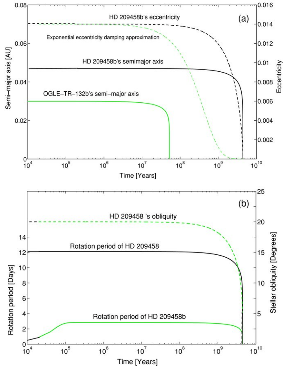
Figure 2. from Falling Transiting Extrasolar Giant Planets LEVRARD ET AL. 2009 ApJ 692 L9 doi:10.1088/0004-637X/692/1/L9 https://dx.doi.org/10.1088/0004-637X/692/1/L9 © 2009. The American Astronomical Society. All rights reserved.
