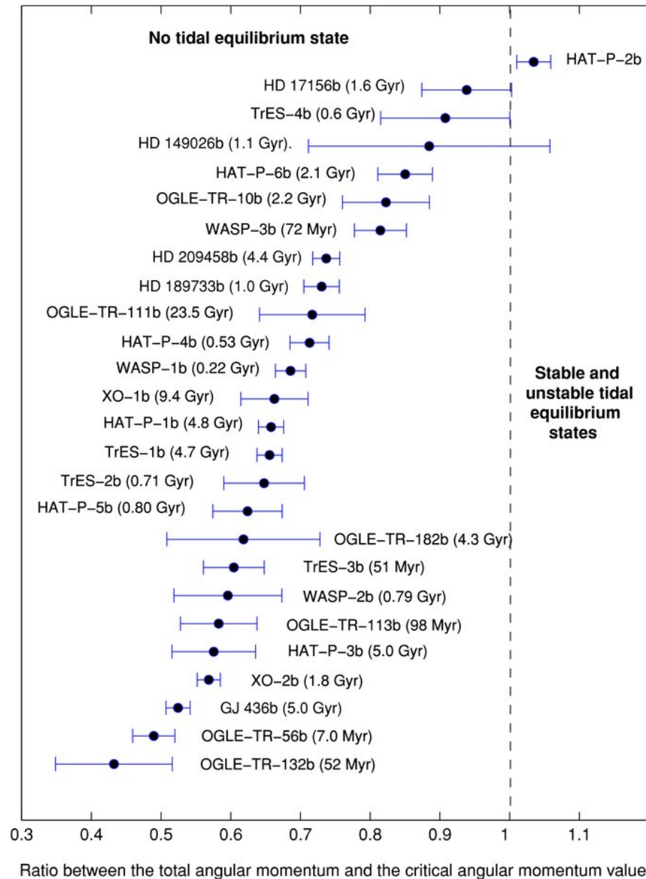
Figure 1. from Falling Transiting Extrasolar Giant Planets LEVRARD ET AL. 2009 ApJ 692 L9 doi:10.1088/0004-637X/692/1/L9 https://dx.doi.org/10.1088/0004-637X/692/1/L9 © 2009. The American Astronomical Society. All rights reserved.
