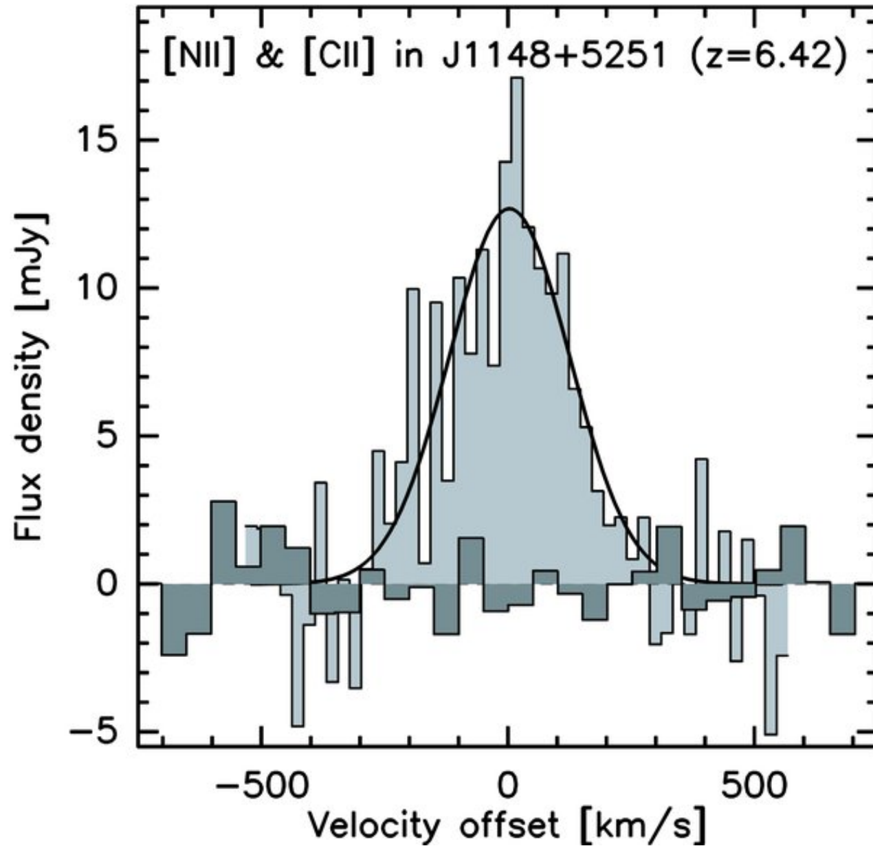
Figure 3. from A Sensitive Search for [N II] \lambda 205 m Emission in a z = 6.4 Quasar Host Galaxy WALTER ET AL. 2009 ApJ 691 L1 doi:10.1088/0004-637X/691/1/L1 https://dx.doi.org/10.1088/0004-637X/691/1/L1 © 2009. The American Astronomical Society. All rights reserved.
