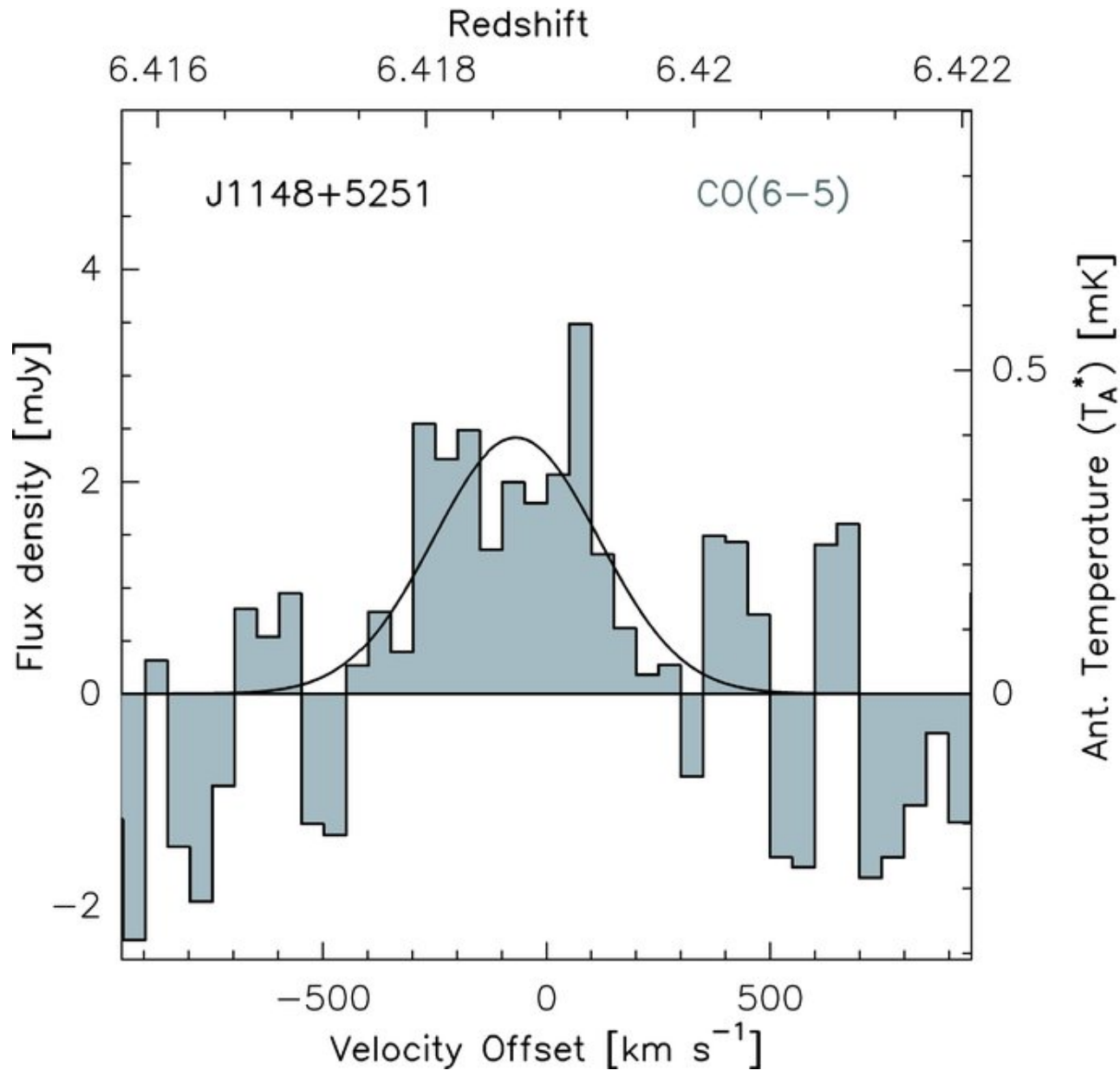
Figure 1. from A Sensitive Search for [N II]205 m Emission in a z = 6.4 Quasar Host Galaxy WALTER ET AL. 2009 ApJ 691 L1 doi:10.1088/0004-637X/691/1/L1 https://dx.doi.org/10.1088/0004-637X/691/1/L1 © 2009. The American Astronomical Society. All rights reserved.
