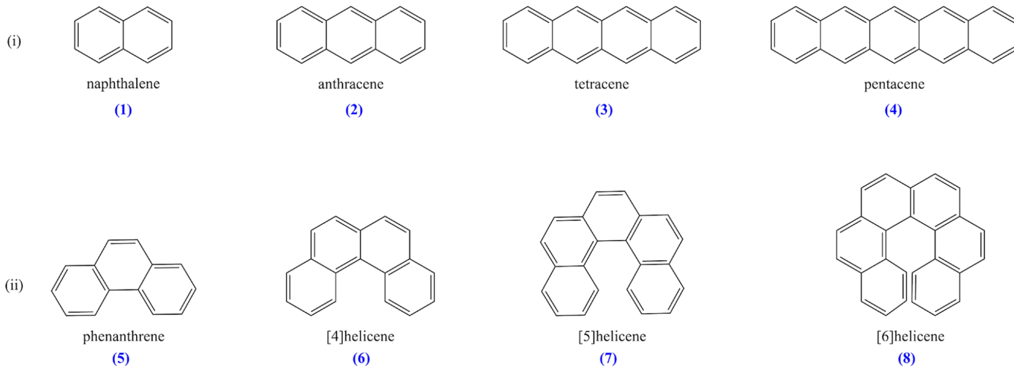
Figure Scheme 1. from Surajit Metya et al 2026 Astrophys. J. 1010 doi:10.3847/1538-4357/aea41c https://dx.doi.org/10.3847/1538-4357/aea41c © 2026. The Author(s). Published by the American Astronomical Society.
