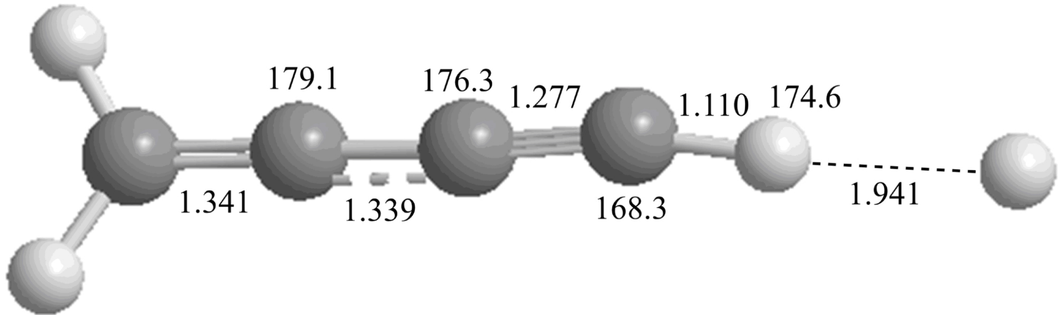
Figure 8. from Surajit Metya et al 2026 Astrophys. J. 1010 doi:10.3847/1538-4357/aea41c https://dx.doi.org/10.3847/1538-4357/aea41c © 2026. The Author(s). Published by the American Astronomical Society.
