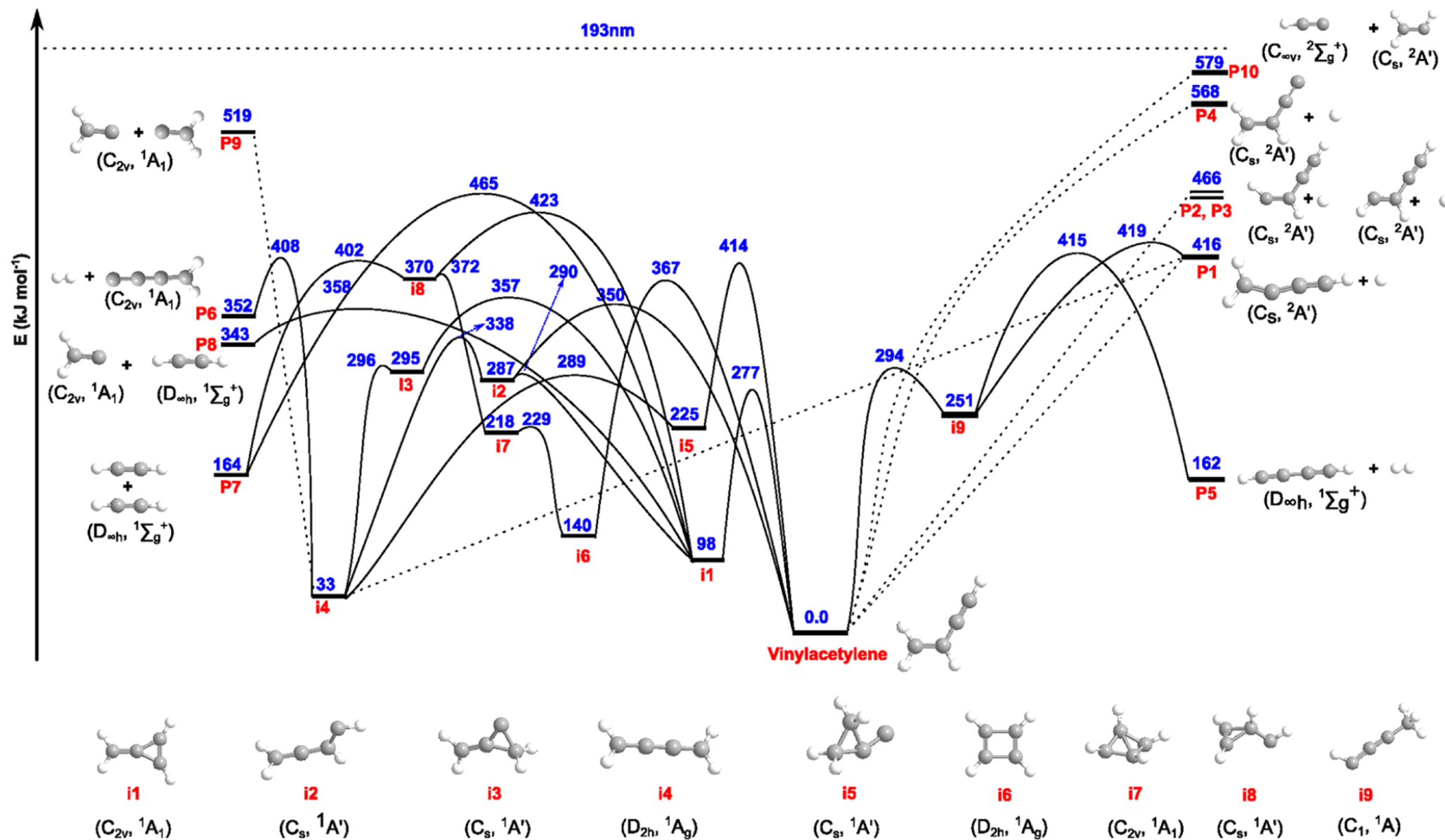
Figure 6. from Surajit Metya et al 2026 Astrophys. J. 1010 doi:10.3847/1538-4357/aea41c https://dx.doi.org/10.3847/1538-4357/aea41c © 2026. The Author(s). Published by the American Astronomical Society.
