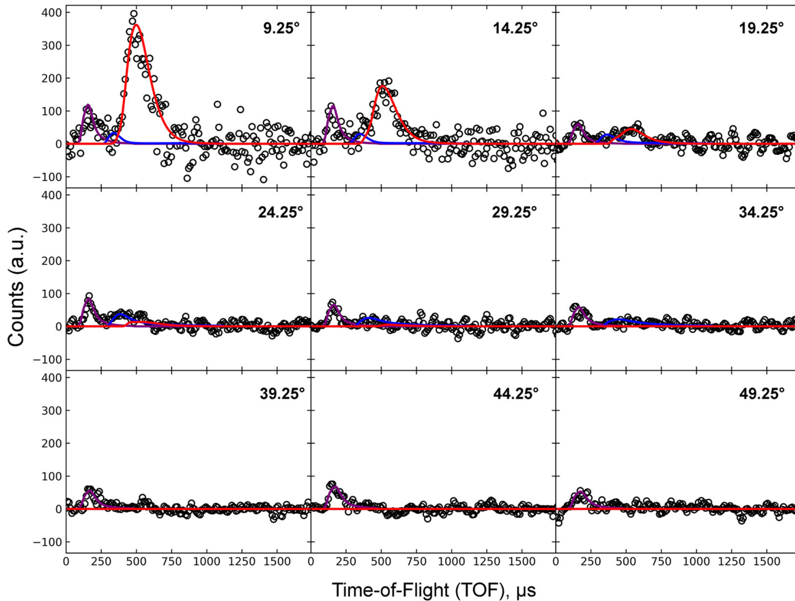
Figure 5. from Surajit Metya et al 2026 Astrophys. J. 1010 doi:10.3847/1538-4357/aea41c https://dx.doi.org/10.3847/1538-4357/aea41c © 2026. The Author(s). Published by the American Astronomical Society.
