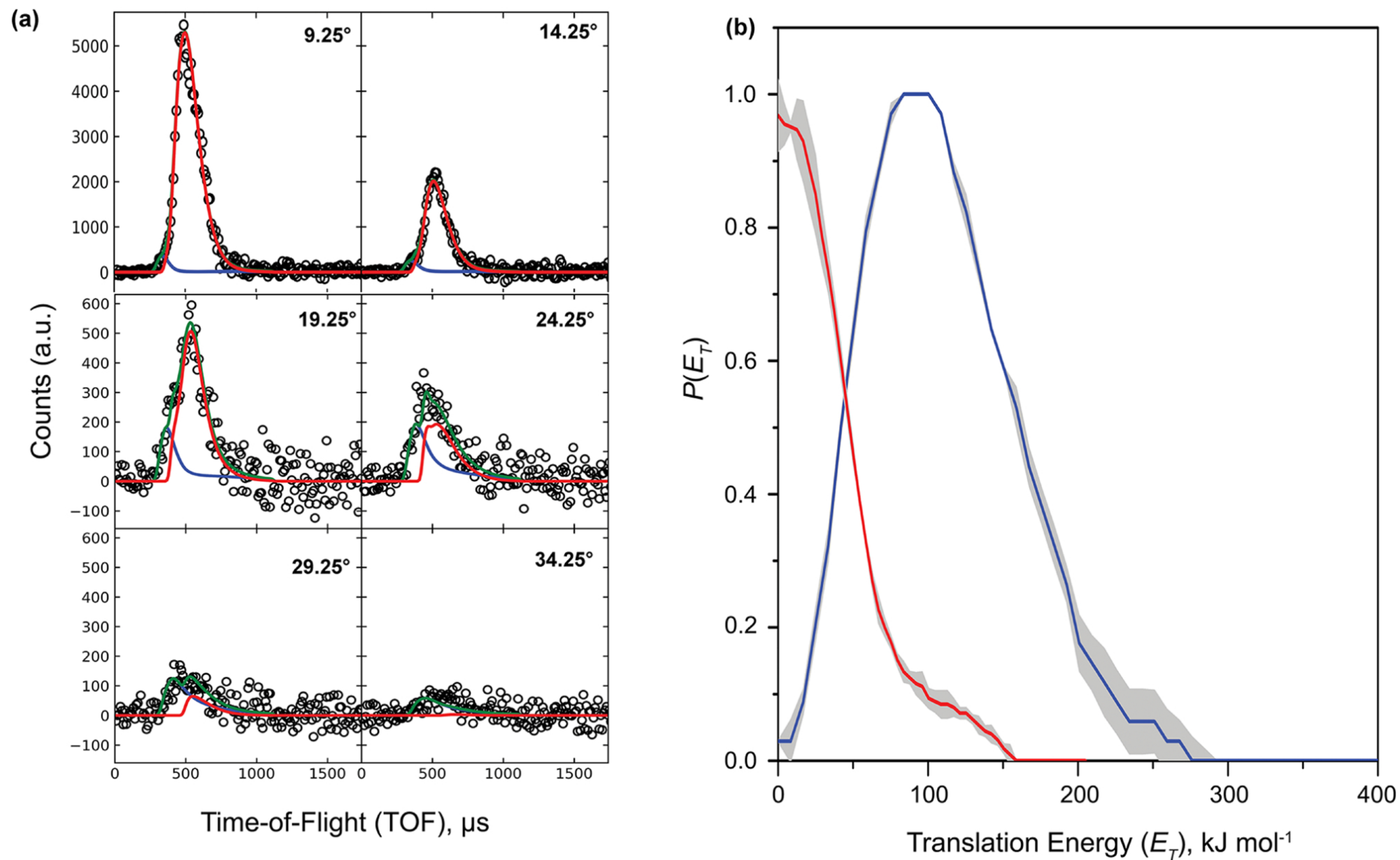
Figure 3. from Surajit Metya et al 2026 Astrophys. J. 1010 doi:10.3847/1538-4357/aea41c https://dx.doi.org/10.3847/1538-4357/aea41c © 2026. The Author(s). Published by the American Astronomical Society.
