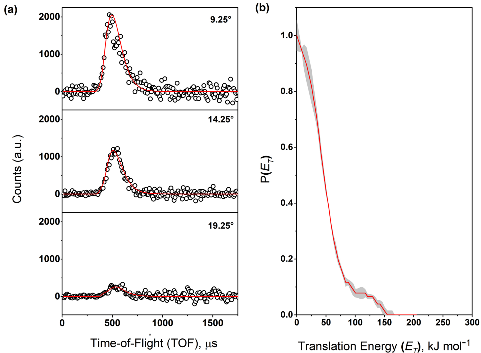
Figure 2. from Surajit Metya et al 2026 Astrophys. J. 1010 doi:10.3847/1538-4357/aea41c https://dx.doi.org/10.3847/1538-4357/aea41c © 2026. The Author(s). Published by the American Astronomical Society.
