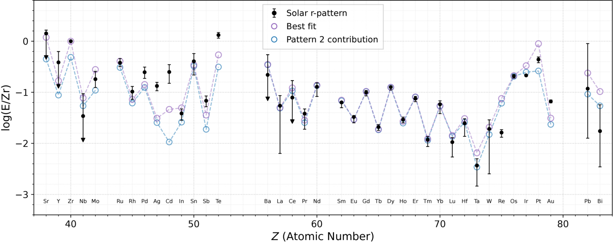
Figure 9. from Chen-Qi Li et al 2026 Astrophys. J. 1010 doi:10.3847/1538-4357/aea137 https://dx.doi.org/10.3847/1538-4357/aea137 © 2026. The Author(s). Published by the American Astronomical Society.
