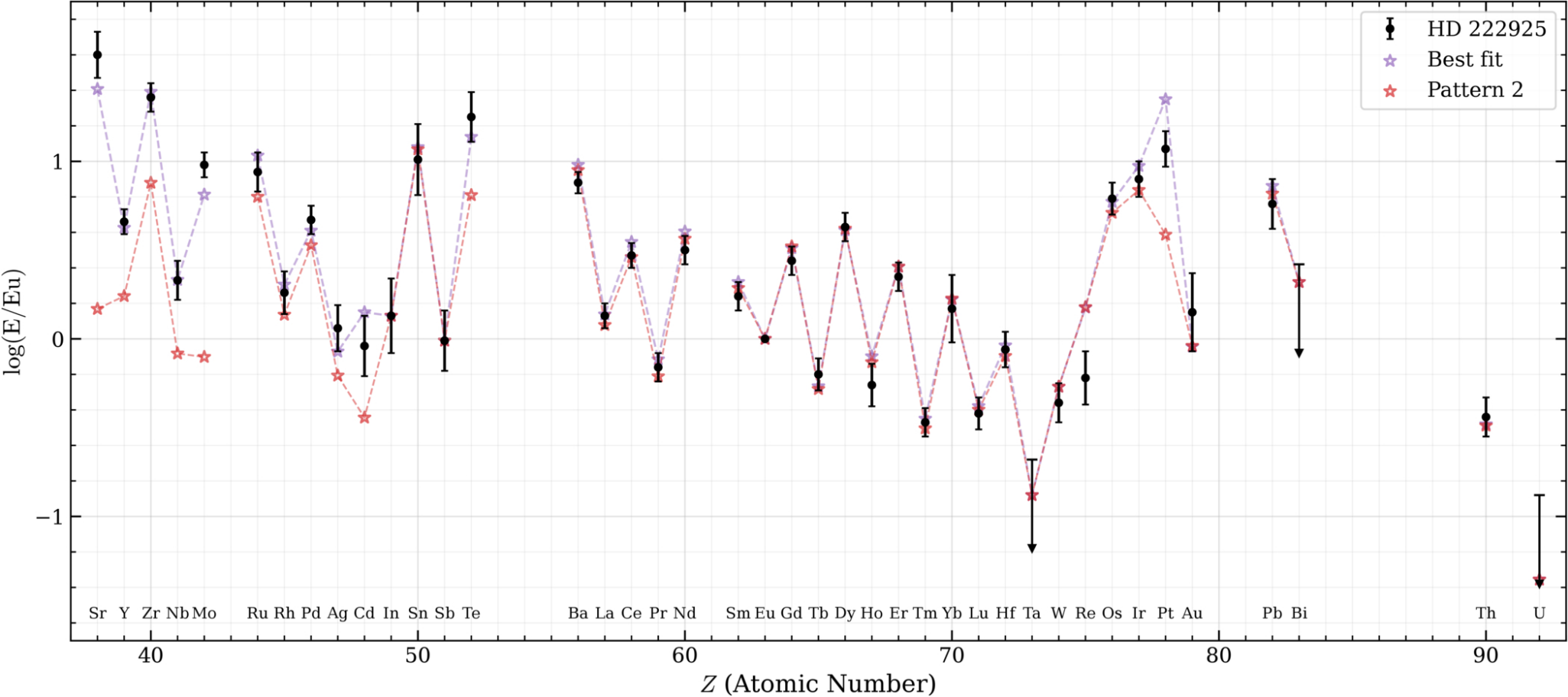
Figure 6. from Chen-Qi Li et al 2026 Astrophys. J. 1010 doi:10.3847/1538-4357/aea137 https://dx.doi.org/10.3847/1538-4357/aea137 © 2026. The Author(s). Published by the American Astronomical Society.
