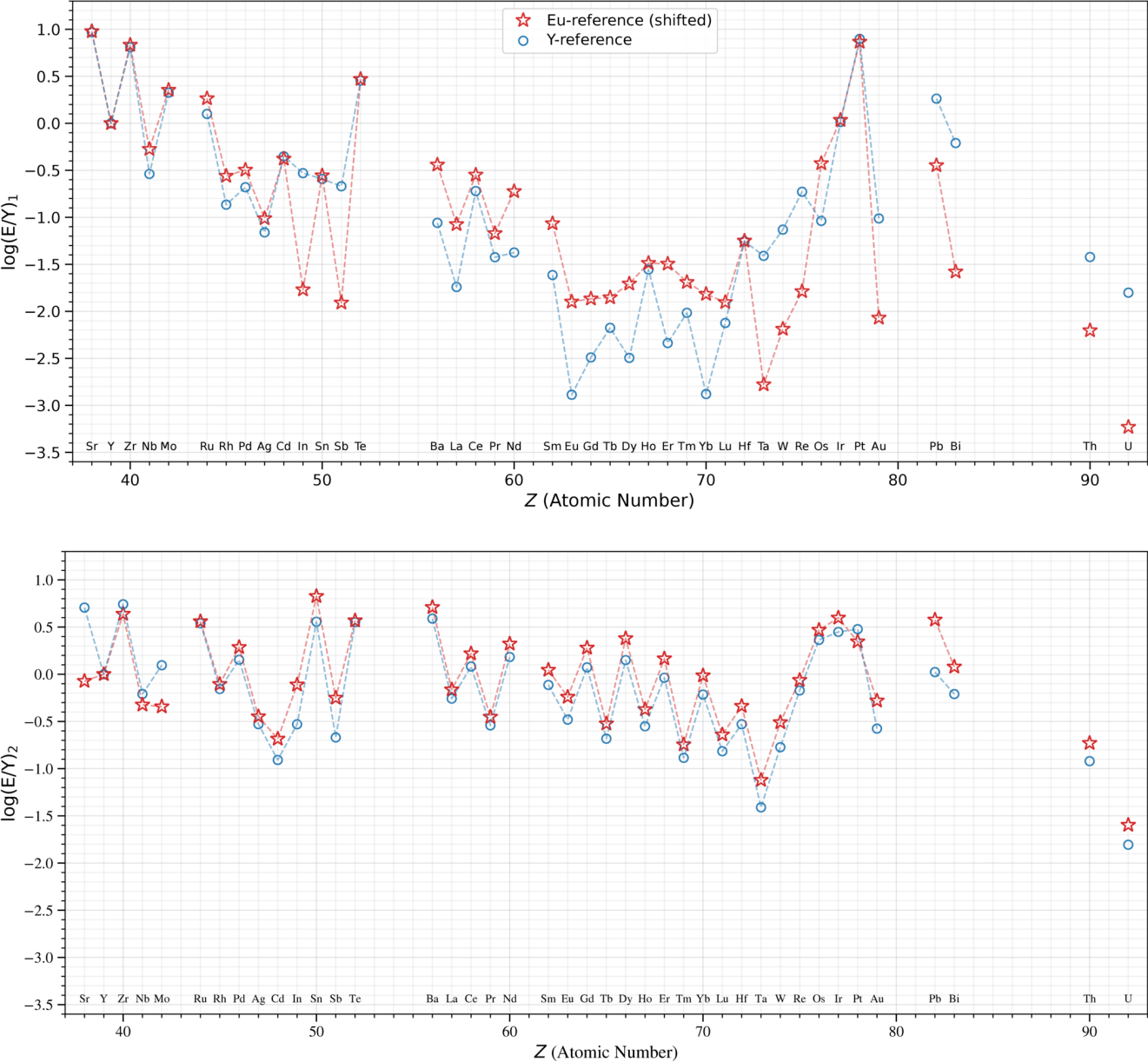
Figure 3. from Chen-Qi Li et al 2026 Astrophys. J. 1010 doi:10.3847/1538-4357/aea137 https://dx.doi.org/10.3847/1538-4357/aea137 © 2026. The Author(s). Published by the American Astronomical Society.
