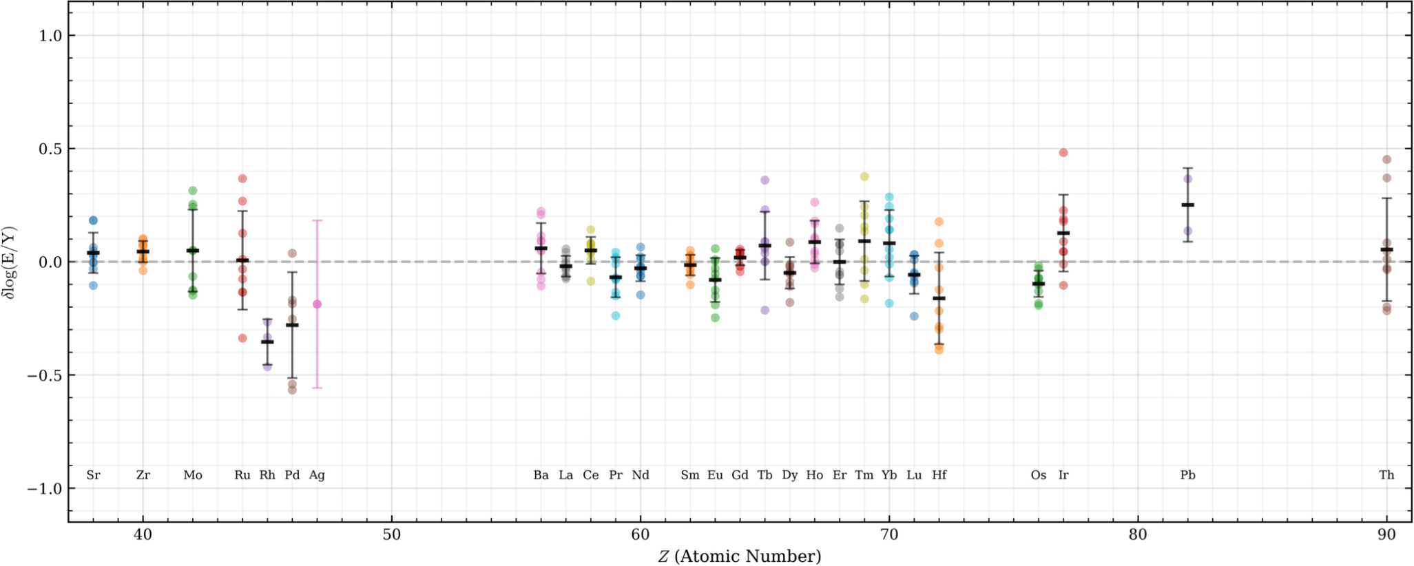
Figure E3. from Chen-Qi Li et al 2026 Astrophys. J. 1010 doi:10.3847/1538-4357/aea137 https://dx.doi.org/10.3847/1538-4357/aea137 © 2026. The Author(s). Published by the American Astronomical Society.
