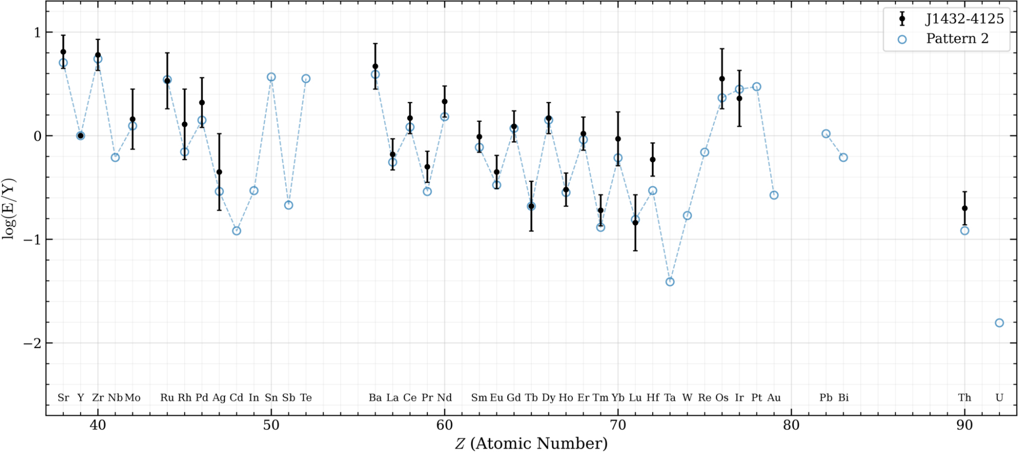
Figure E2. from Chen-Qi Li et al 2026 Astrophys. J. 1010 doi:10.3847/1538-4357/aea137 https://dx.doi.org/10.3847/1538-4357/aea137 © 2026. The Author(s). Published by the American Astronomical Society.
