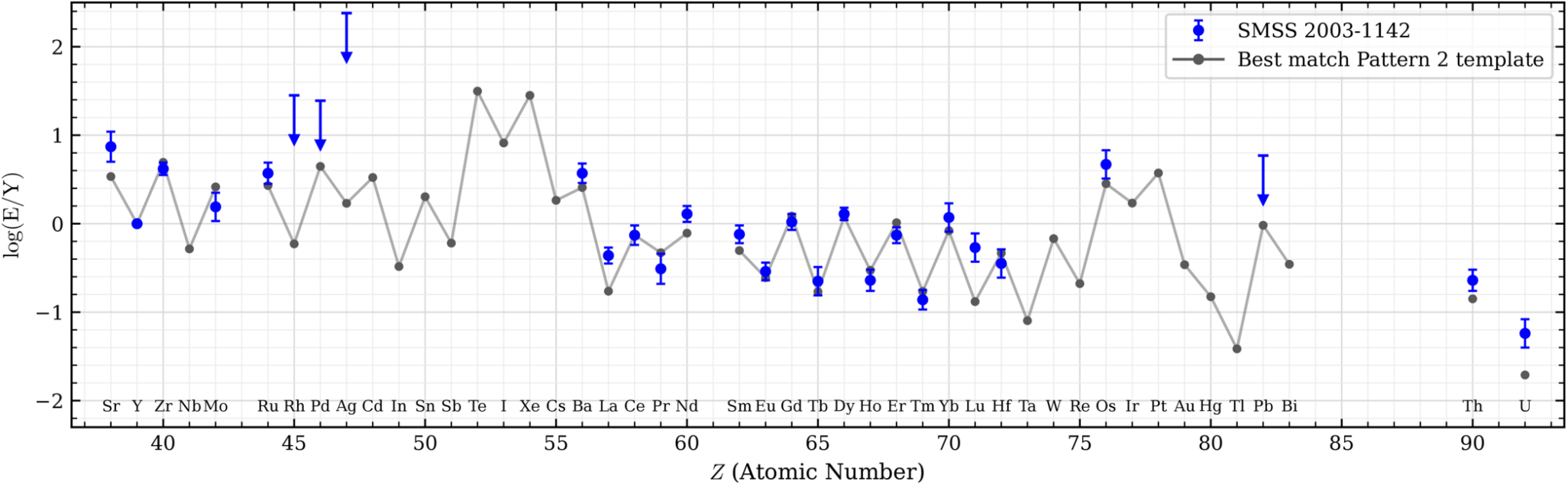
Figure 11. from Chen-Qi Li et al 2026 Astrophys. J. 1010 doi:10.3847/1538-4357/aea137 https://dx.doi.org/10.3847/1538-4357/aea137 © 2026. The Author(s). Published by the American Astronomical Society.
