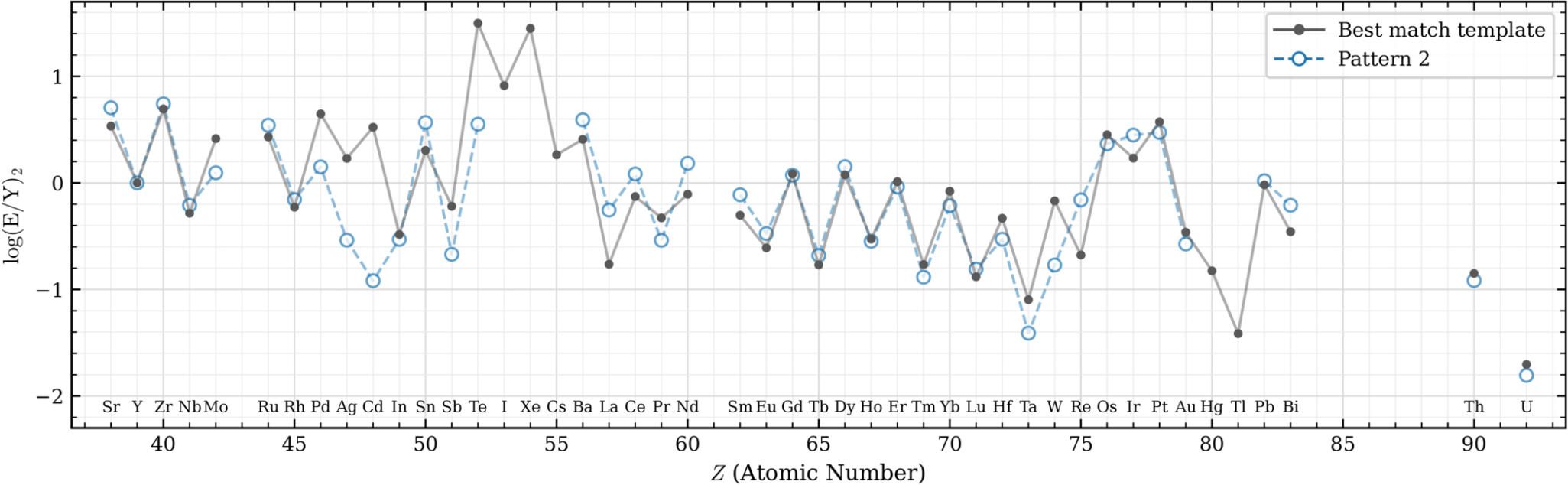
Figure 10. from Chen-Qi Li et al 2026 Astrophys. J. 1010 doi:10.3847/1538-4357/aea137 https://dx.doi.org/10.3847/1538-4357/aea137 © 2026. The Author(s). Published by the American Astronomical Society.
