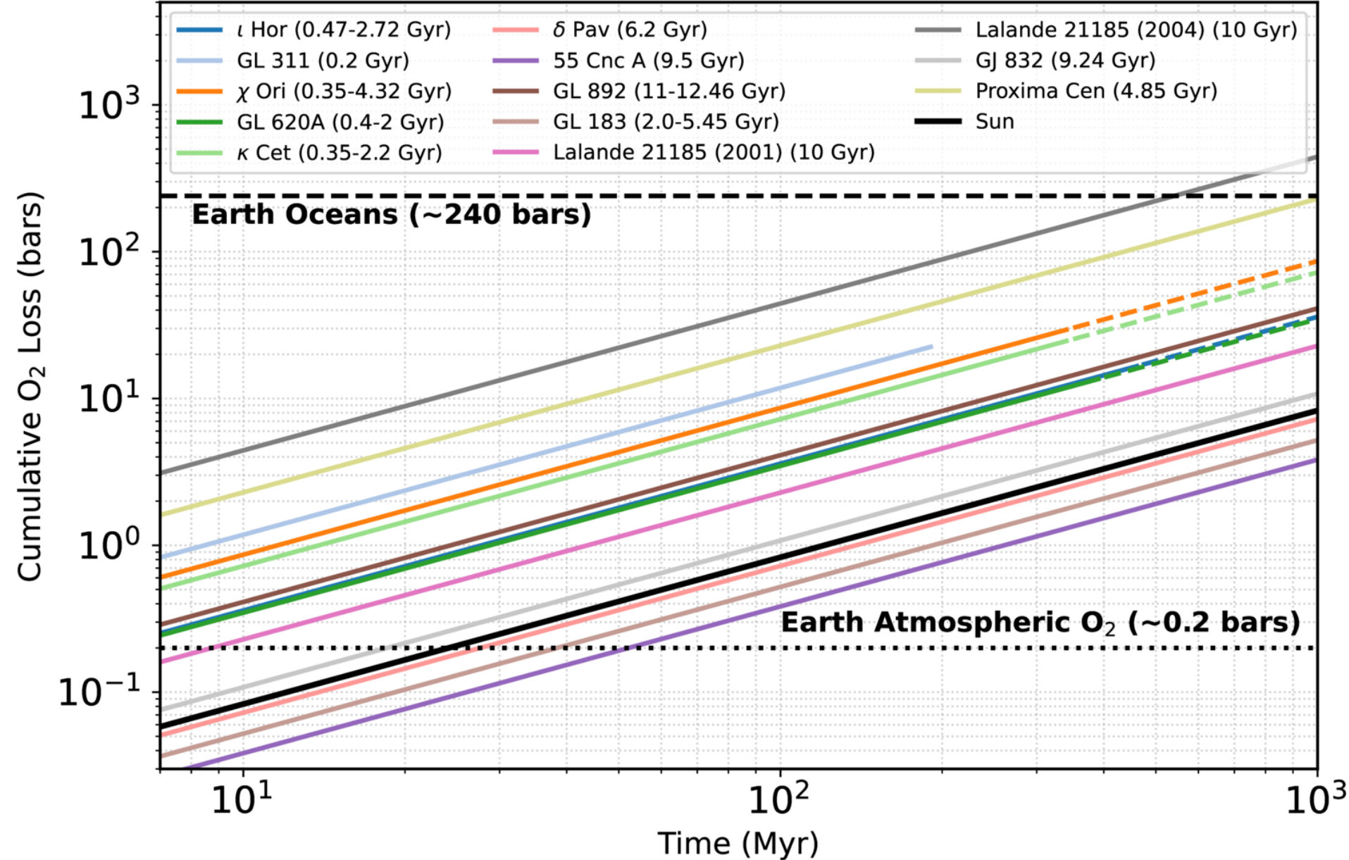
Figure 8. from Sarah Peacock et al 2026 Astrophys. J. 1009 doi:10.3847/1538-4357/aea076 https://dx.doi.org/10.3847/1538-4357/aea076 © 2026. The Author(s). Published by the American Astronomical Society.
